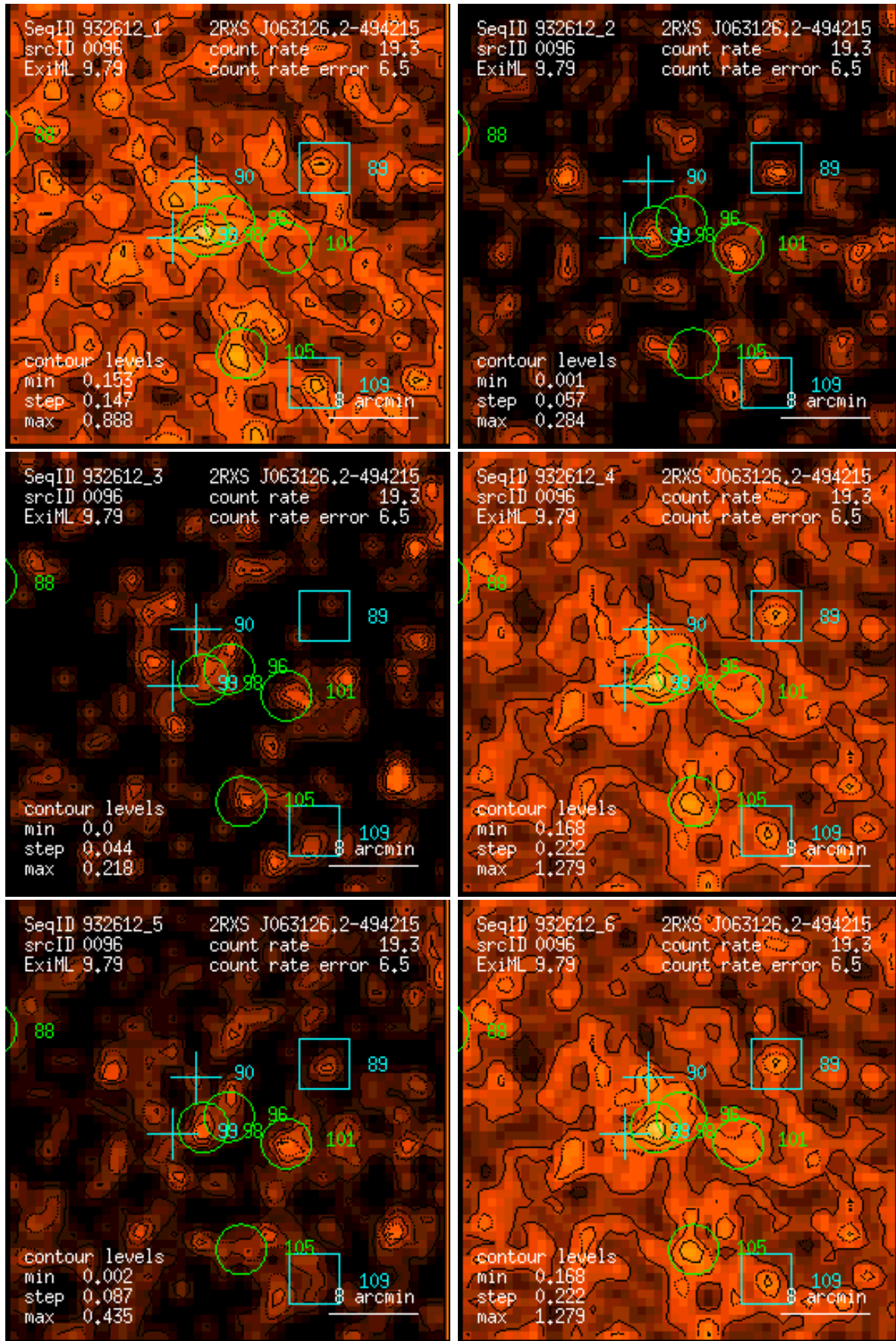
Figure 96: RASS 932612: detection 0096: band rate images, Gaussian filter: (1) PSPC channels 11 – 41, (2) 52 – 90, (3) 91 – 201, (4) 11 – 235, (5) 52 – 201, (6) 11 – 201. Broad band rates in counts/ks. Band rate contour levels in counts/ks/arcmin 2 .
