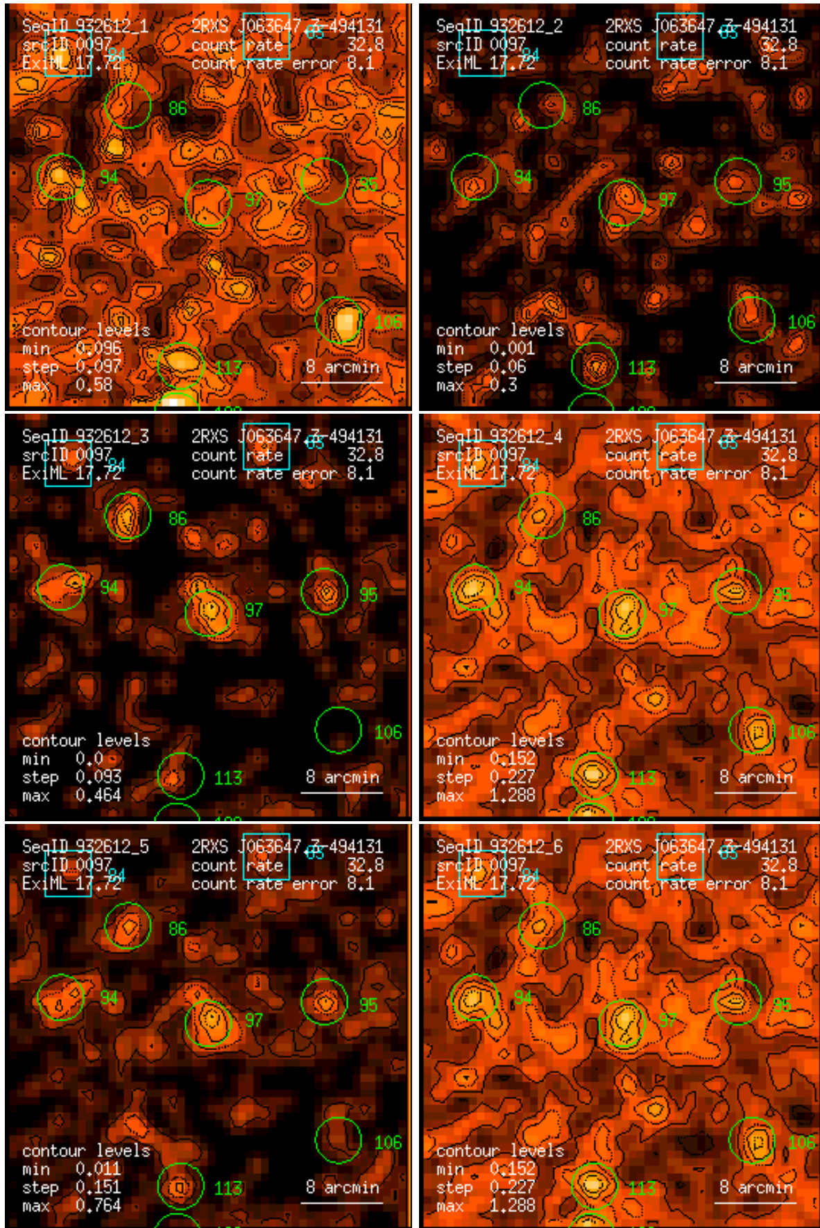
Figure 97: RASS 932612: detection 0097: band rate images, Gaussian filter: (1) PSPC channels 11 – 41, (2) 52 – 90, (3) 91 – 201, (4) 11 – 235, (5) 52 – 201, (6) 11 – 201. Broad band rates in counts/ks. Band rate contour levels in counts/ks/arcmin 2 .
