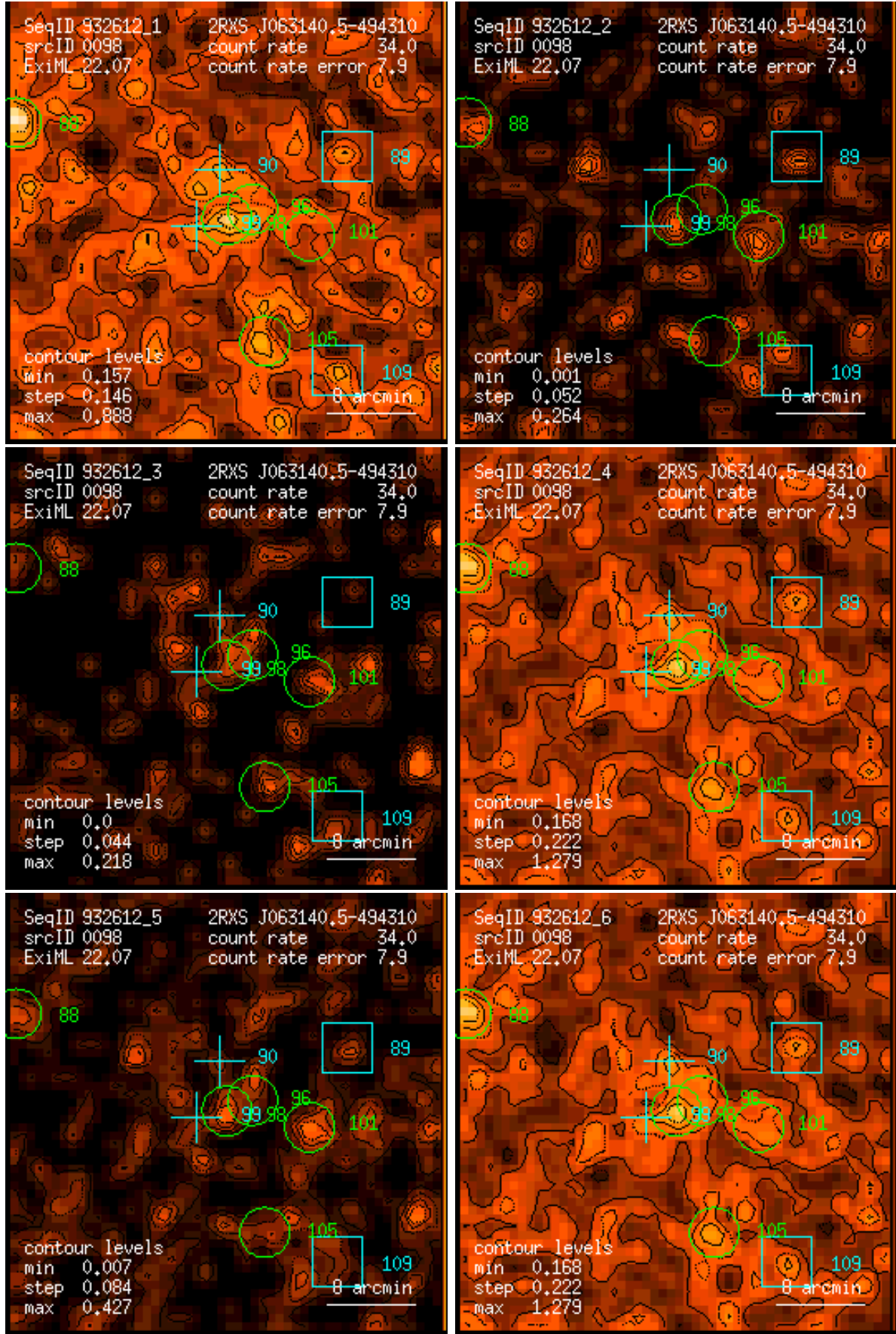
Figure 98: RASS 932612: detection 0098: band rate images, Gaussian filter: (1) PSPC channels 11 – 41, (2) 52 – 90, (3) 91 – 201, (4) 11 – 235, (5) 52 – 201, (6) 11 – 201. Broad band rates in counts/ks. Band rate contour levels in counts/ks/arcmin 2 .
