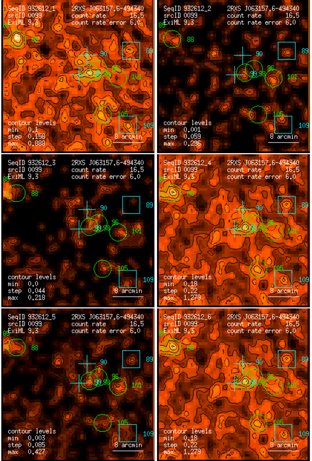
Figure 99: RASS 932612: detection 0099: band rate images, Gaussian filter: (1) PSPC channels 11 – 41, (2) 52 – 90, (3) 91 – 201, (4) 11 – 235, (5) 52 – 201, (6) 11 – 201. Broad band rates in counts/ks. Band rate contour levels in counts/ks/arcmin 2 .
