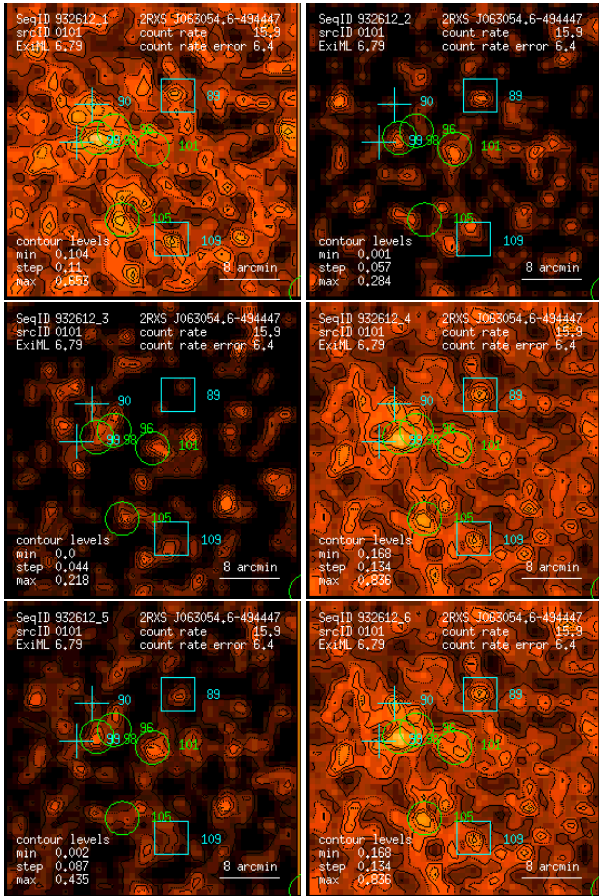
Figure 101: RASS 932612: detection 0101: band rate images, Gaussian filter: (1) PSPC channels 11 – 41, (2) 52 – 90, (3) 91 – 201, (4) 11 – 235, (5) 52 – 201, (6) 11 – 201. Broad band rates in counts/ks. Band rate contour levels in counts/ks/arcmin 2 .
