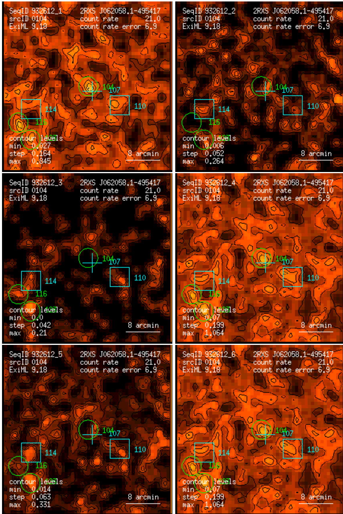
Figure 104: RASS 932612: detection 0104: band rate images, Gaussian filter: (1) PSPC channels 11 – 41, (2) 52 – 90, (3) 91 – 201, (4) 11 – 235, (5) 52 – 201, (6) 11 – 201. Broad band rates in counts/ks. Band rate contour levels in counts/ks/arcmin 2 .
