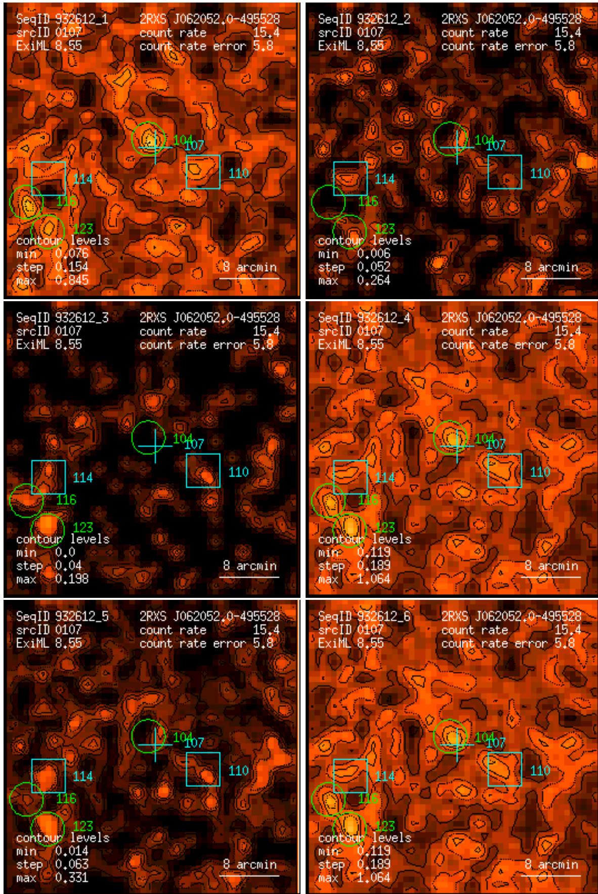
Figure 107: RASS 932612: detection 0107: band rate images, Gaussian filter: (1) PSPC channels 11 – 41, (2) 52 – 90, (3) 91 – 201, (4) 11 – 235, (5) 52 – 201, (6) 11 – 201. Broad band rates in counts/ks. Band rate contour levels in counts/ks/arcmin 2 .
