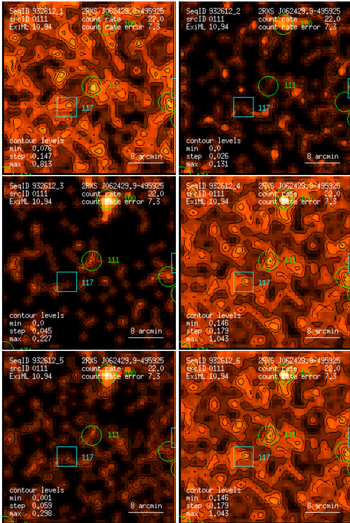
Figure 111: RASS 932612: detection 0111: band rate images, Gaussian filter: (1) PSPC channels 11 – 41, (2) 52 – 90, (3) 91 – 201, (4) 11 – 235, (5) 52 – 201, (6) 11 – 201. Broad band rates in counts/ks. Band rate contour levels in counts/ks/arcmin 2 .
