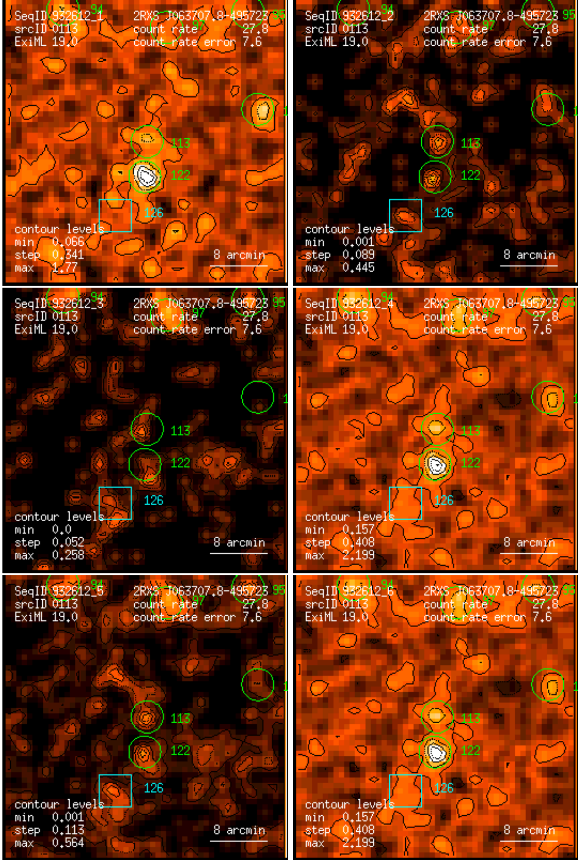
Figure 113: RASS 932612: detection 0113: band rate images, Gaussian filter: (1) PSPC channels 11 – 41, (2) 52 – 90, (3) 91 – 201, (4) 11 – 235, (5) 52 – 201, (6) 11 – 201. Broad band rates in counts/ks. Band rate contour levels in counts/ks/arcmin 2 .
