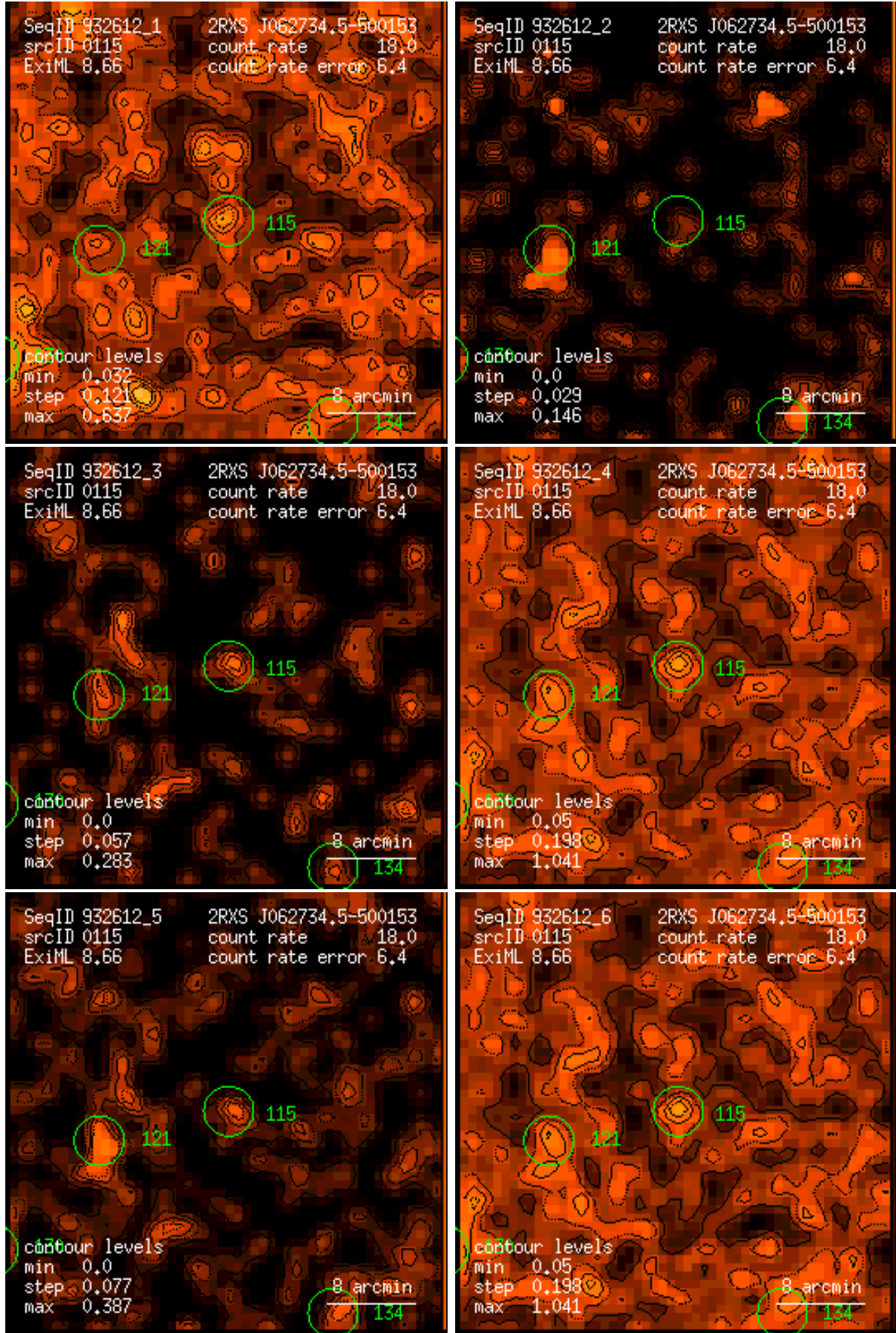
Figure 115: RASS 932612: detection 0115: band rate images, Gaussian filter: (1) PSPC channels 11 – 41, (2) 52 – 90, (3) 91 – 201, (4) 11 – 235, (5) 52 – 201, (6) 11 – 201. Broad band rates in counts/ks. Band rate contour levels in counts/ks/arcmin 2 .
