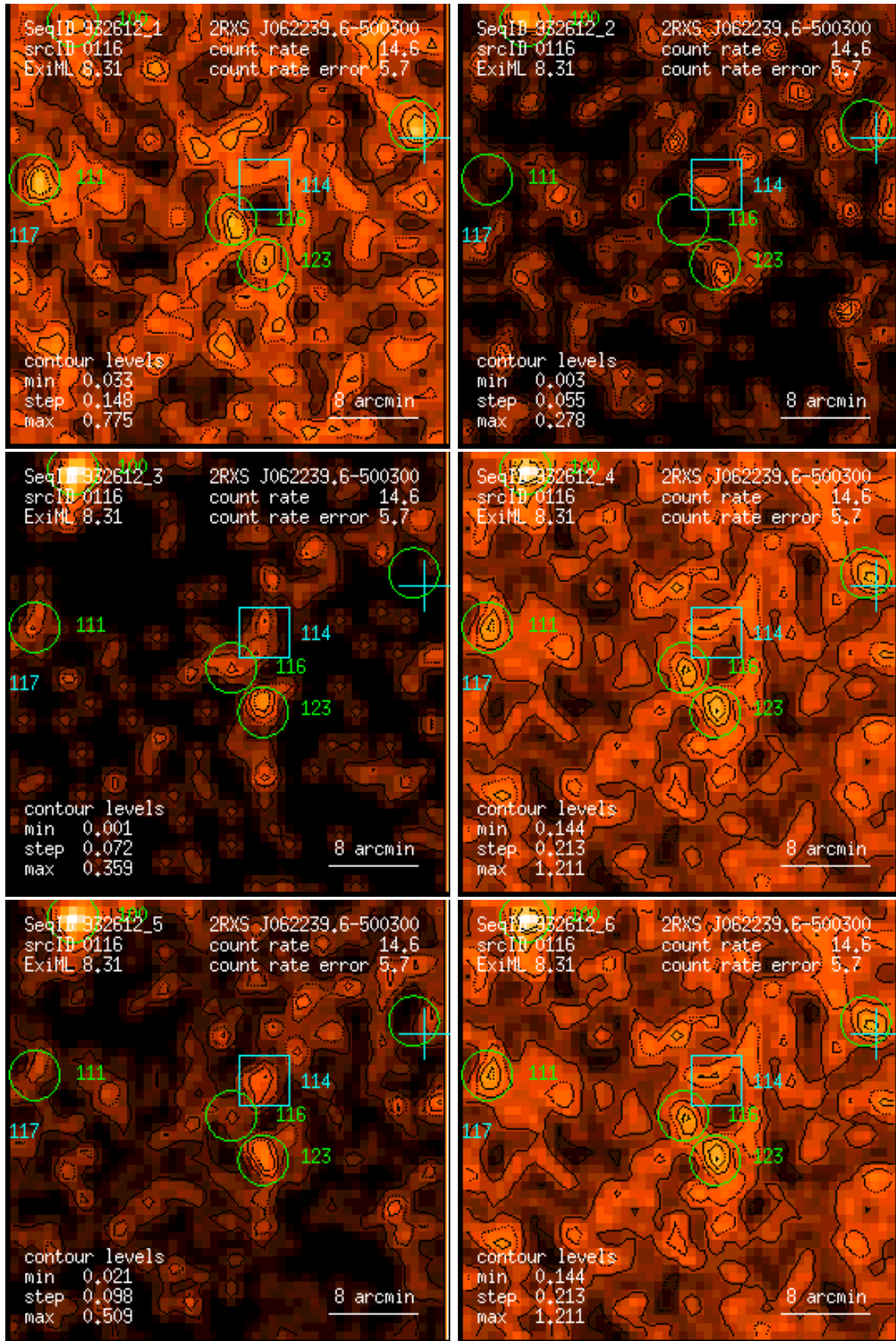
Figure 116: RASS 932612: detection 0116: band rate images, Gaussian filter: (1) PSPC channels 11 – 41, (2) 52 – 90, (3) 91 – 201, (4) 11 – 235, (5) 52 – 201, (6) 11 – 201. Broad band rates in counts/ks. Band rate contour levels in counts/ks/arcmin 2 .
