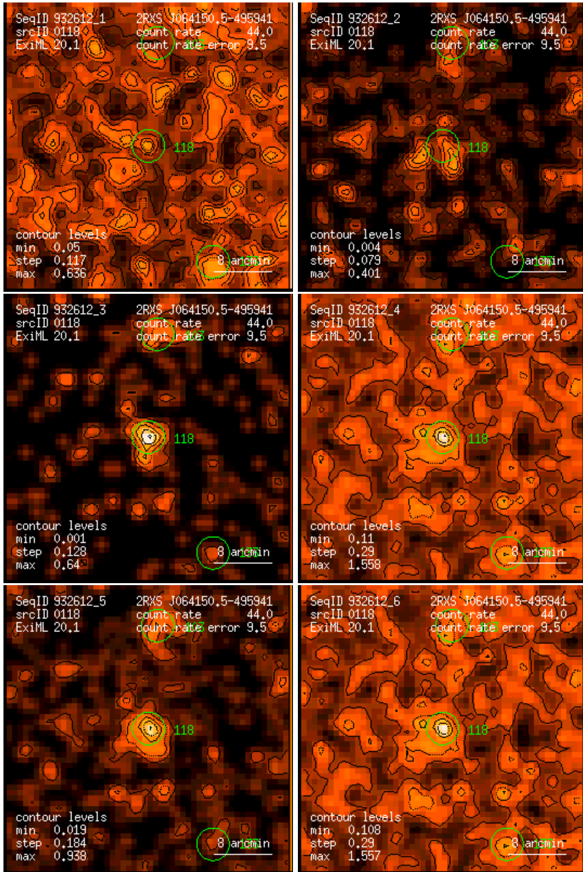
Figure 118: RASS 932612: detection 0118: band rate images, Gaussian filter: (1) PSPC channels 11 – 41, (2) 52 – 90, (3) 91 – 201, (4) 11 – 235, (5) 52 – 201, (6) 11 – 201. Broad band rates in counts/ks. Band rate contour levels in counts/ks/arcmin 2 .
