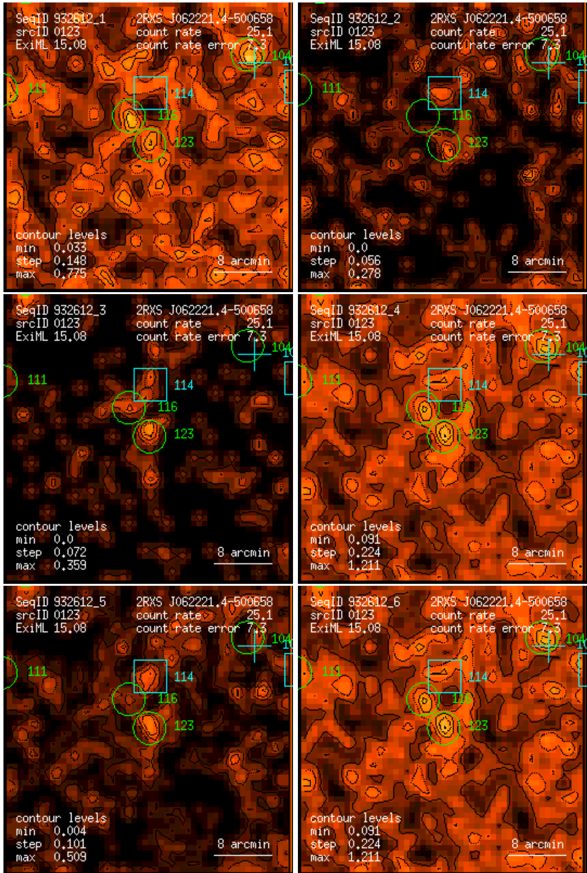
Figure 123: RASS 932612: detection 0123: band rate images, Gaussian filter: (1) PSPC channels 11 – 41, (2) 52 – 90, (3) 91 – 201, (4) 11 – 235, (5) 52 – 201, (6) 11 – 201. Broad band rates in counts/ks. Band rate contour levels in counts/ks/arcmin 2 .
