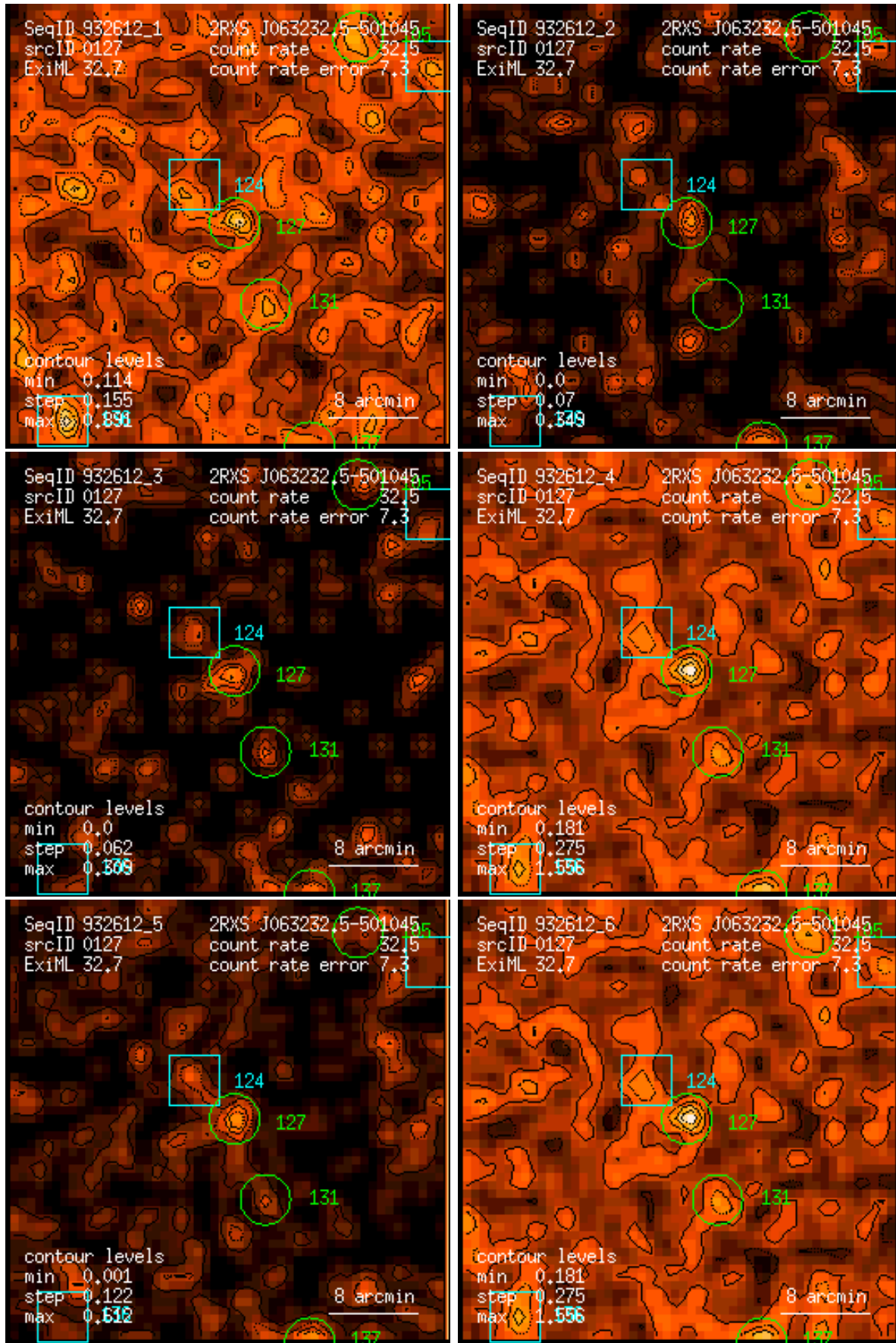
Figure 127: RASS 932612: detection 0127: band rate images, Gaussian filter: (1) PSPC channels 11 – 41, (2) 52 – 90, (3) 91 – 201, (4) 11 – 235, (5) 52 – 201, (6) 11 – 201. Broad band rates in counts/ks. Band rate contour levels in counts/ks/arcmin 2 .
