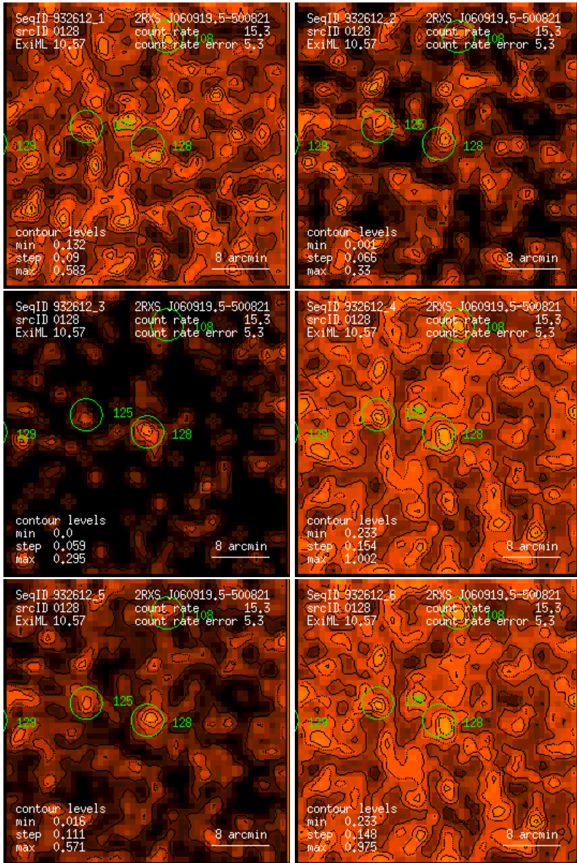
Figure 128: RASS 932612: detection 0128: band rate images, Gaussian filter: (1) PSPC channels 11 – 41, (2) 52 – 90, (3) 91 – 201, (4) 11 – 235, (5) 52 – 201, (6) 11 – 201. Broad band rates in counts/ks. Band rate contour levels in counts/ks/arcmin 2 .
