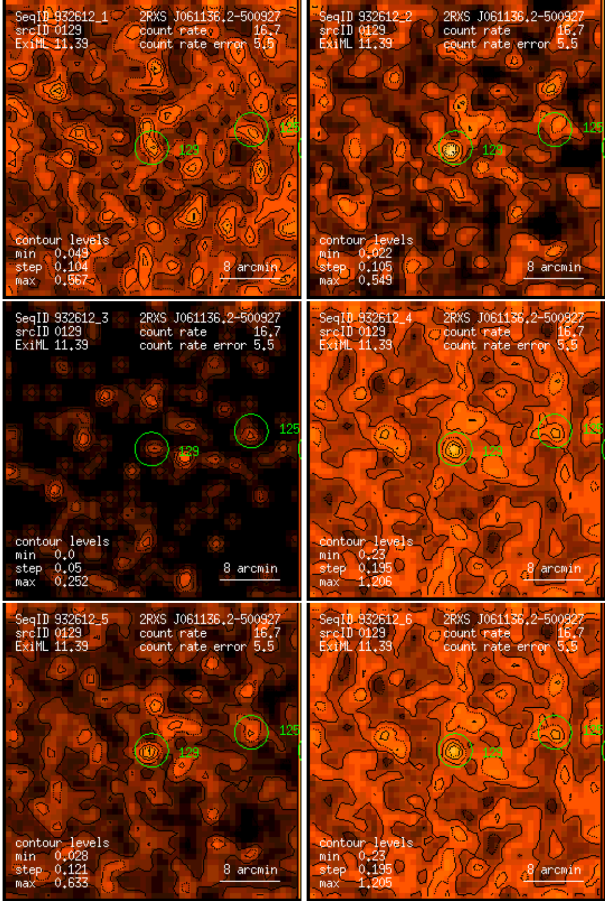
Figure 129: RASS 932612: detection 0129: band rate images, Gaussian filter: (1) PSPC channels 11 – 41, (2) 52 – 90, (3) 91 – 201, (4) 11 – 235, (5) 52 – 201, (6) 11 – 201. Broad band rates in counts/ks. Band rate contour levels in counts/ks/arcmin 2 .
