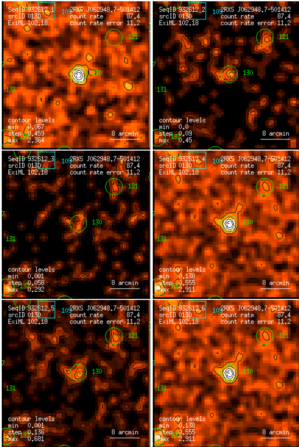
Figure 130: RASS 932612: detection 0130: band rate images, Gaussian filter: (1) PSPC channels 11 – 41, (2) 52 – 90, (3) 91 – 201, (4) 11 – 235, (5) 52 – 201, (6) 11 – 201. Broad band rates in counts/ks. Band rate contour levels in counts/ks/arcmin 2 .
