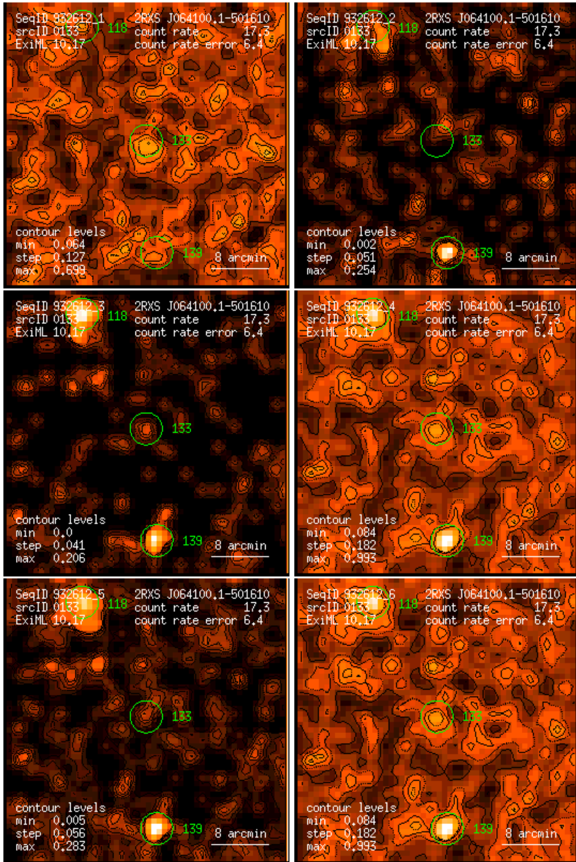
Figure 133: RASS 932612: detection 0133: band rate images, Gaussian filter: (1) PSPC channels 11 – 41, (2) 52 – 90, (3) 91 – 201, (4) 11 – 235, (5) 52 – 201, (6) 11 – 201. Broad band rates in counts/ks. Band rate contour levels in counts/ks/arcmin 2 .
