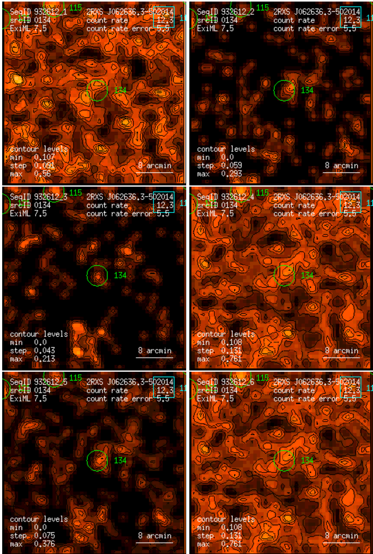
Figure 134: RASS 932612: detection 0134: band rate images, Gaussian filter: (1) PSPC channels 11 – 41, (2) 52 – 90, (3) 91 – 201, (4) 11 – 235, (5) 52 – 201, (6) 11 – 201. Broad band rates in counts/ks. Band rate contour levels in counts/ks/arcmin 2 .
