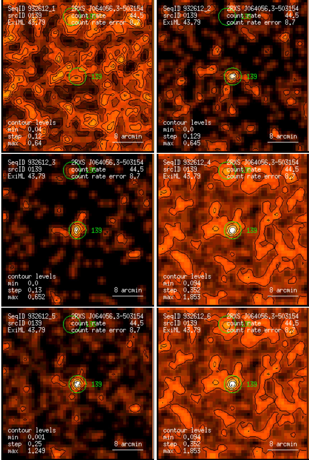
Figure 139: RASS 932612: detection 0139: band rate images, Gaussian filter: (1) PSPC channels 11 – 41, (2) 52 – 90, (3) 91 – 201, (4) 11 – 235, (5) 52 – 201, (6) 11 – 201. Broad band rates in counts/ks. Band rate contour levels in counts/ks/arcmin 2 .
