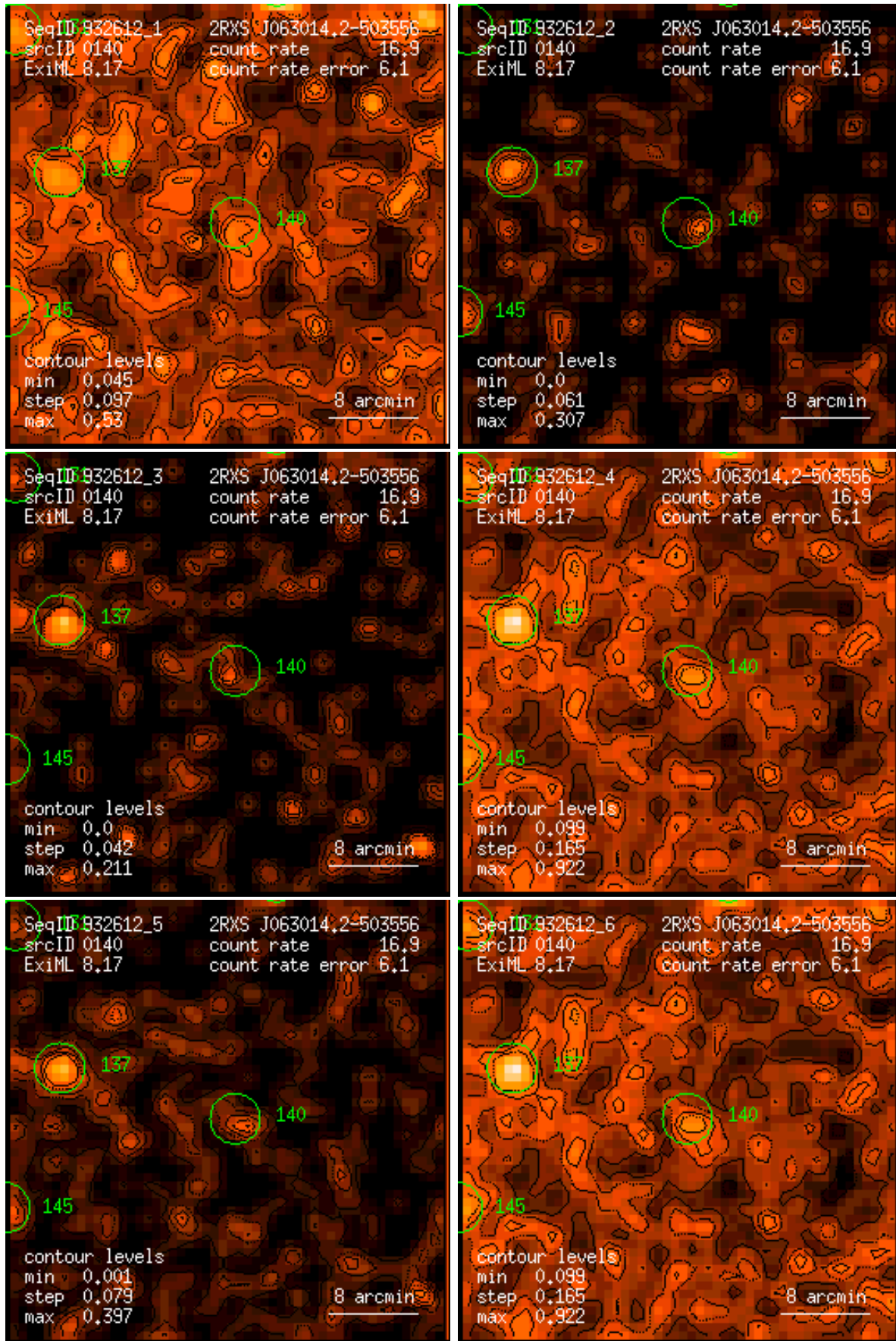
Figure 140: RASS 932612: detection 0140: band rate images, Gaussian filter: (1) PSPC channels 11 – 41, (2) 52 – 90, (3) 91 – 201, (4) 11 – 235, (5) 52 – 201, (6) 11 – 201. Broad band rates in counts/ks. Band rate contour levels in counts/ks/arcmin 2 .
