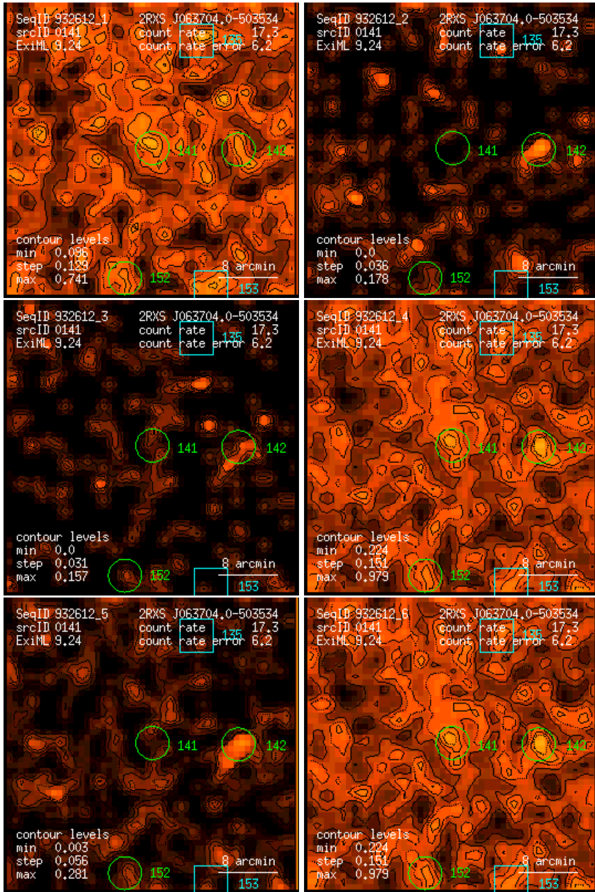
Figure 141: RASS 932612: detection 0141: band rate images, Gaussian filter: (1) PSPC channels 11 – 41, (2) 52 – 90, (3) 91 – 201, (4) 11 – 235, (5) 52 – 201, (6) 11 – 201. Broad band rates in counts/ks. Band rate contour levels in counts/ks/arcmin 2 .
