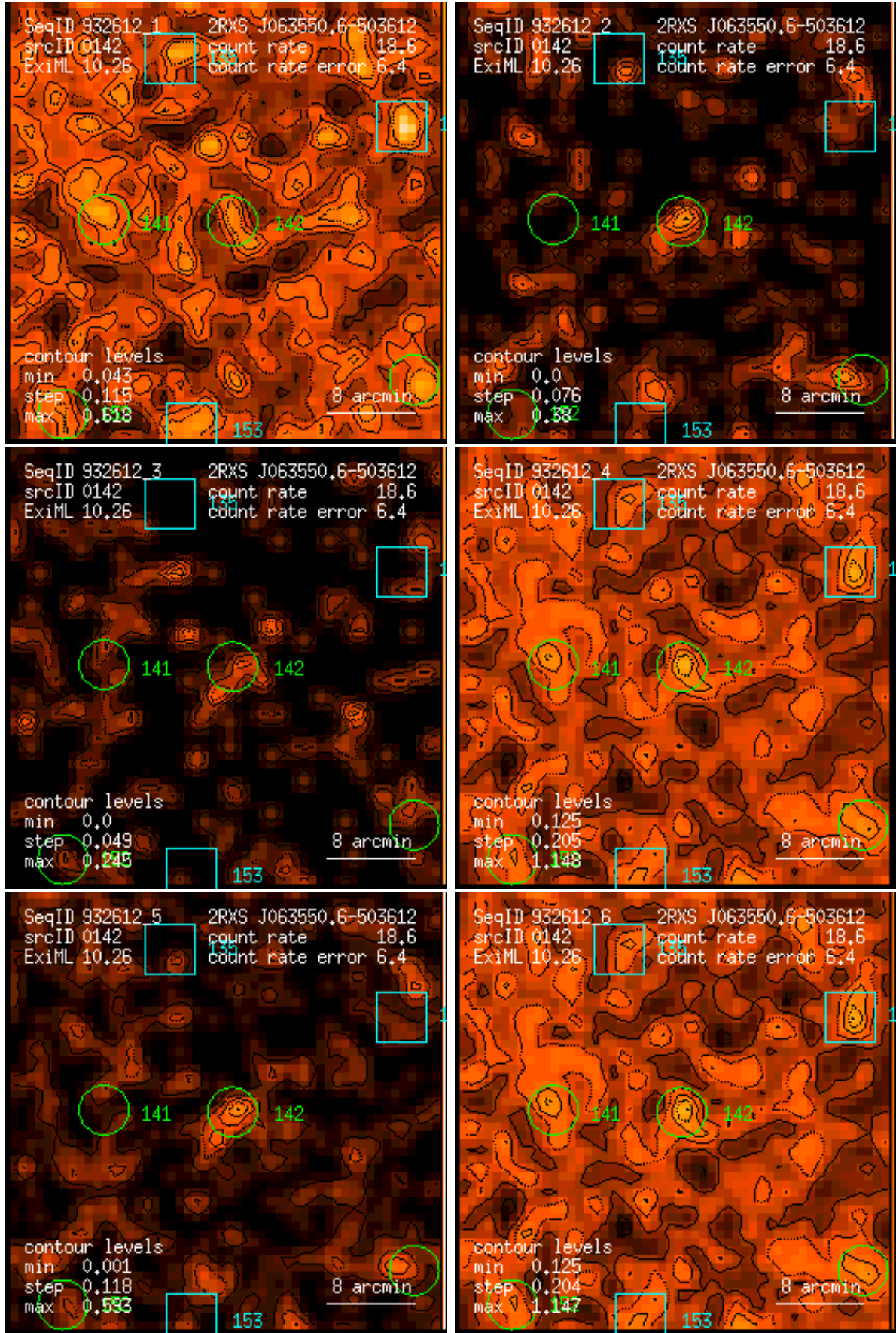
Figure 142: RASS 932612: detection 0142: band rate images, Gaussian filter: (1) PSPC channels 11 – 41, (2) 52 – 90, (3) 91 – 201, (4) 11 – 235, (5) 52 – 201, (6) 11 – 201. Broad band rates in counts/ks. Band rate contour levels in counts/ks/arcmin 2 .
