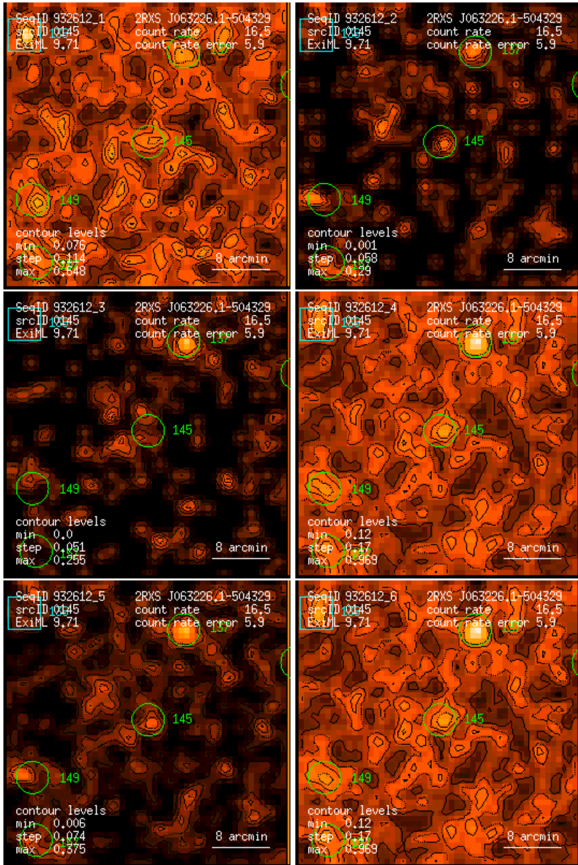
Figure 145: RASS 932612: detection 0145: band rate images, Gaussian filter: (1) PSPC channels 11 – 41, (2) 52 – 90, (3) 91 – 201, (4) 11 – 235, (5) 52 – 201, (6) 11 – 201. Broad band rates in counts/ks. Band rate contour levels in counts/ks/arcmin 2 .
