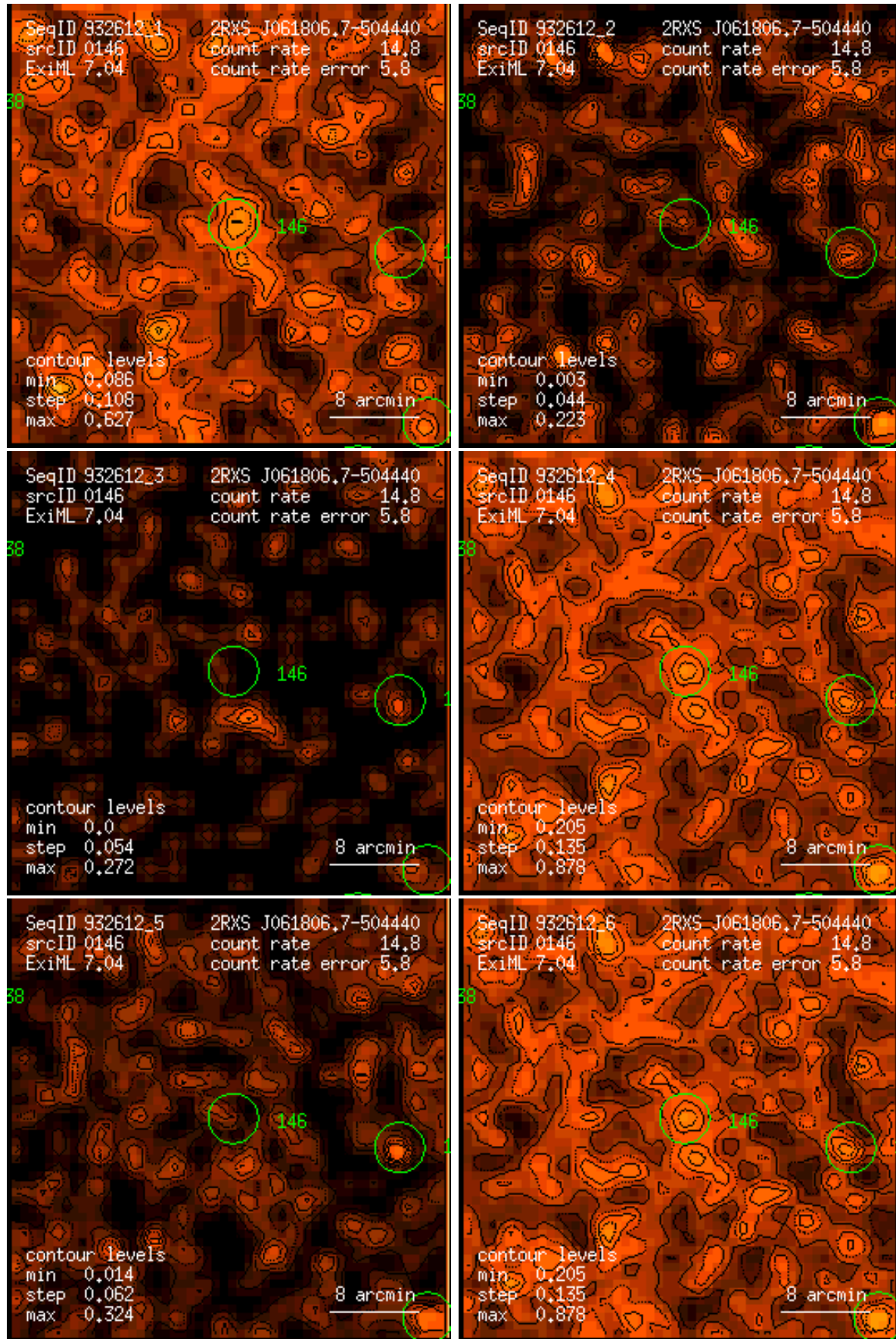
Figure 146: RASS 932612: detection 0146: band rate images, Gaussian filter: (1) PSPC channels 11 – 41, (2) 52 – 90, (3) 91 – 201, (4) 11 – 235, (5) 52 – 201, (6) 11 – 201. Broad band rates in counts/ks. Band rate contour levels in counts/ks/arcmin 2 .
