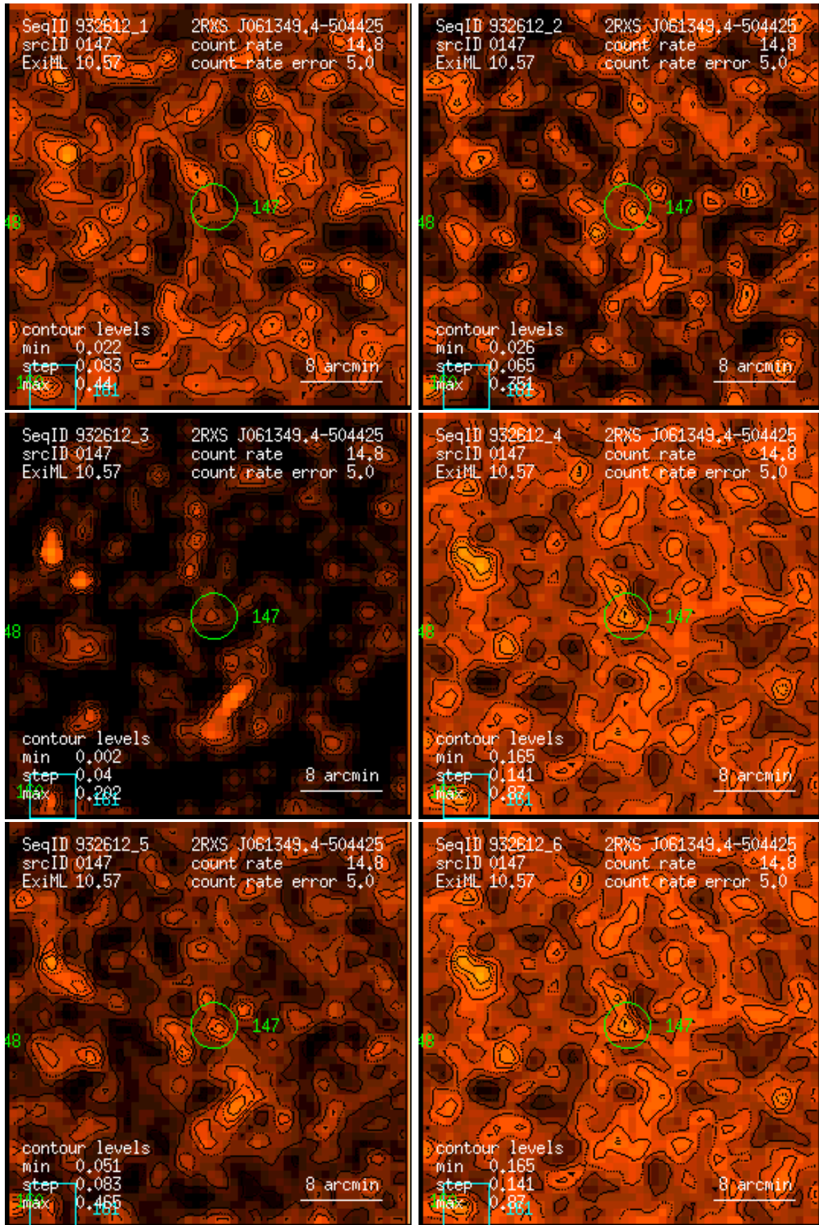
Figure 147: RASS 932612: detection 0147: band rate images, Gaussian filter: (1) PSPC channels 11 – 41, (2) 52 – 90, (3) 91 – 201, (4) 11 – 235, (5) 52 – 201, (6) 11 – 201. Broad band rates in counts/ks. Band rate contour levels in counts/ks/arcmin 2 .
