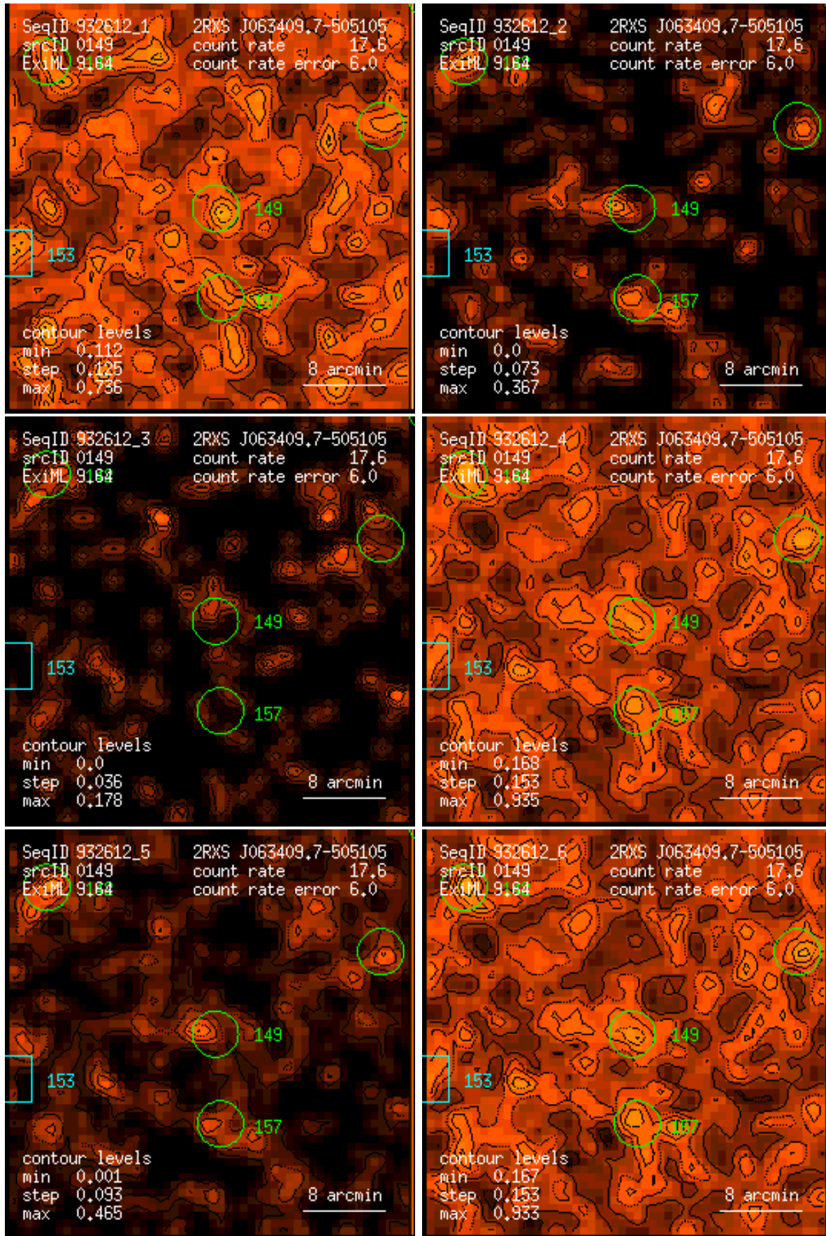
Figure 149: RASS 932612: detection 0149: band rate images, Gaussian filter: (1) PSPC channels 11 – 41, (2) 52 – 90, (3) 91 – 201, (4) 11 – 235, (5) 52 – 201, (6) 11 – 201. Broad band rates in counts/ks. Band rate contour levels in counts/ks/arcmin 2 .
