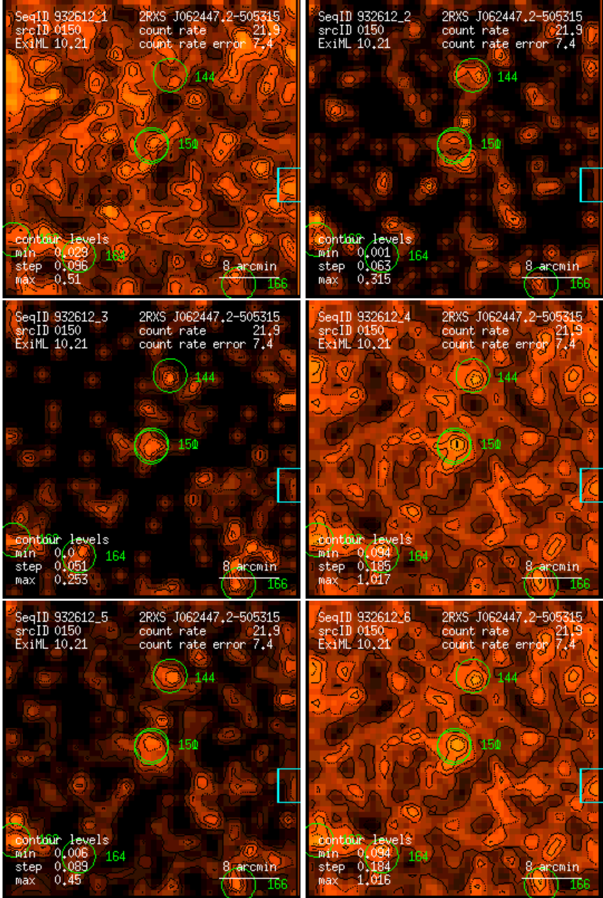
Figure 150: RASS 932612: detection 0150: band rate images, Gaussian filter: (1) PSPC channels 11 – 41, (2) 52 – 90, (3) 91 – 201, (4) 11 – 235, (5) 52 – 201, (6) 11 – 201. Broad band rates in counts/ks. Band rate contour levels in counts/ks/arcmin 2 .
