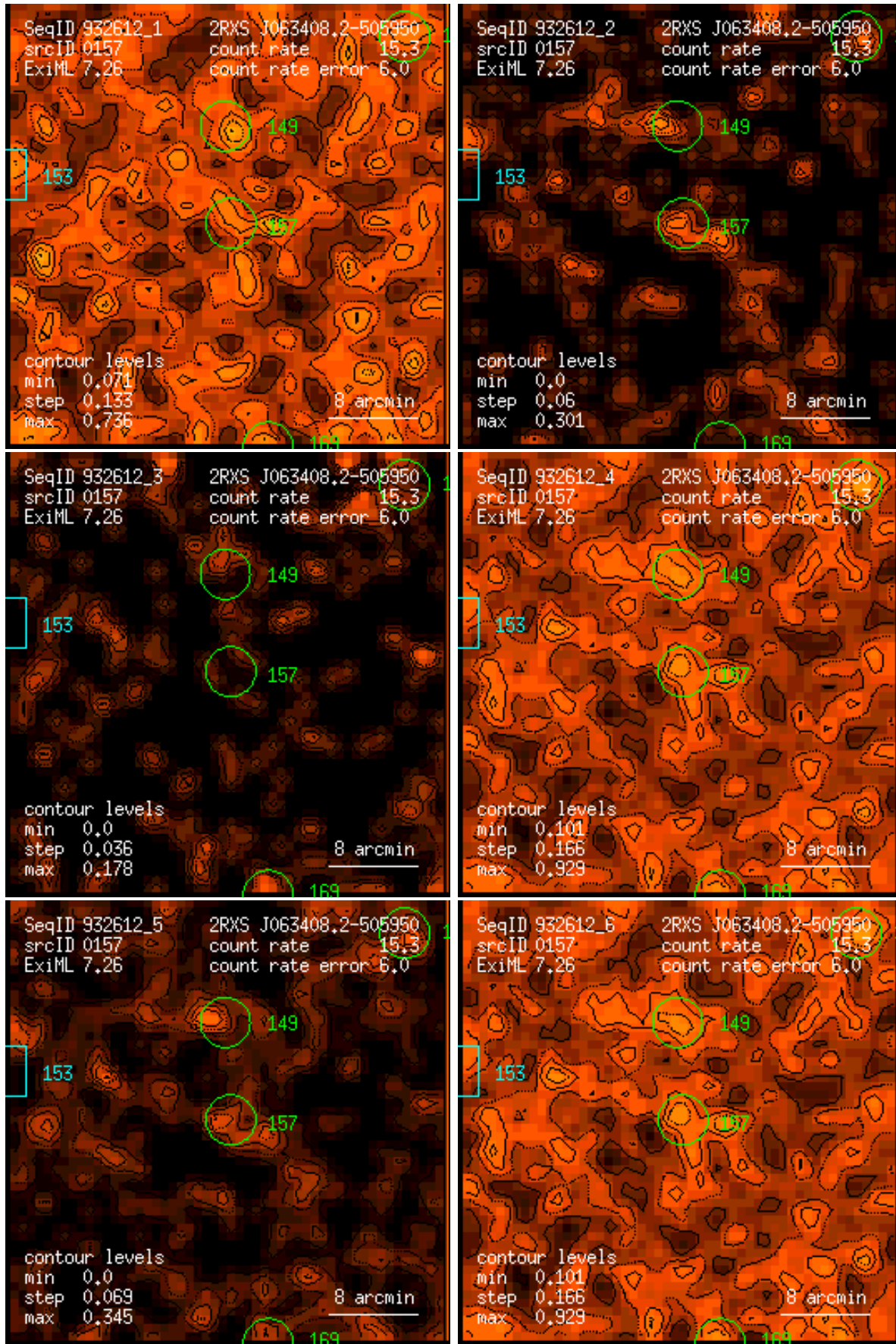
Figure 157: RASS 932612: detection 0157: band rate images, Gaussian filter: (1) PSPC channels 11 – 41, (2) 52 – 90, (3) 91 – 201, (4) 11 – 235, (5) 52 – 201, (6) 11 – 201. Broad band rates in counts/ks. Band rate contour levels in counts/ks/arcmin 2 .
