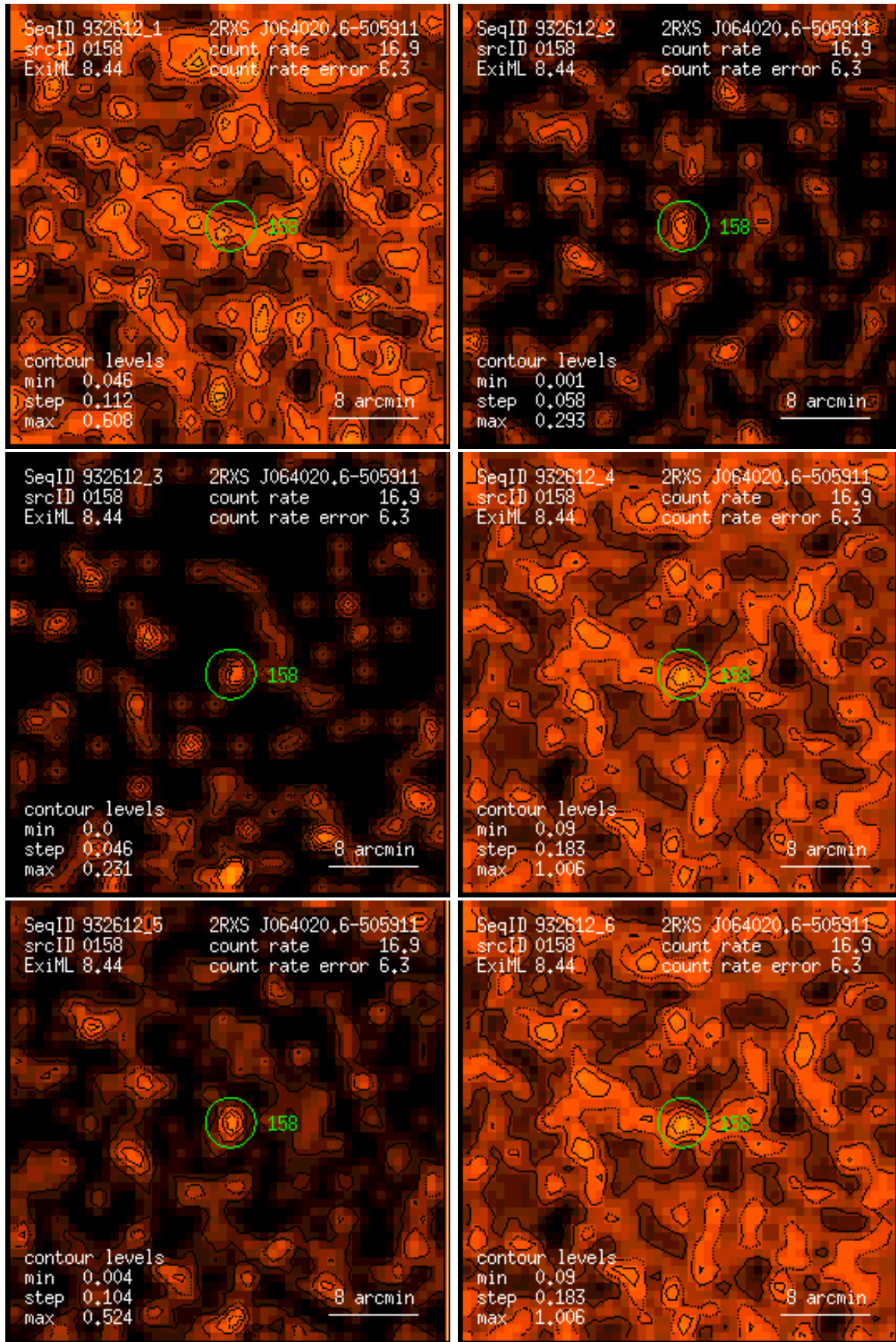
Figure 158: RASS 932612: detection 0158: band rate images, Gaussian filter: (1) PSPC channels 11 – 41, (2) 52 – 90, (3) 91 – 201, (4) 11 – 235, (5) 52 – 201, (6) 11 – 201. Broad band rates in counts/ks. Band rate contour levels in counts/ks/arcmin 2 .
