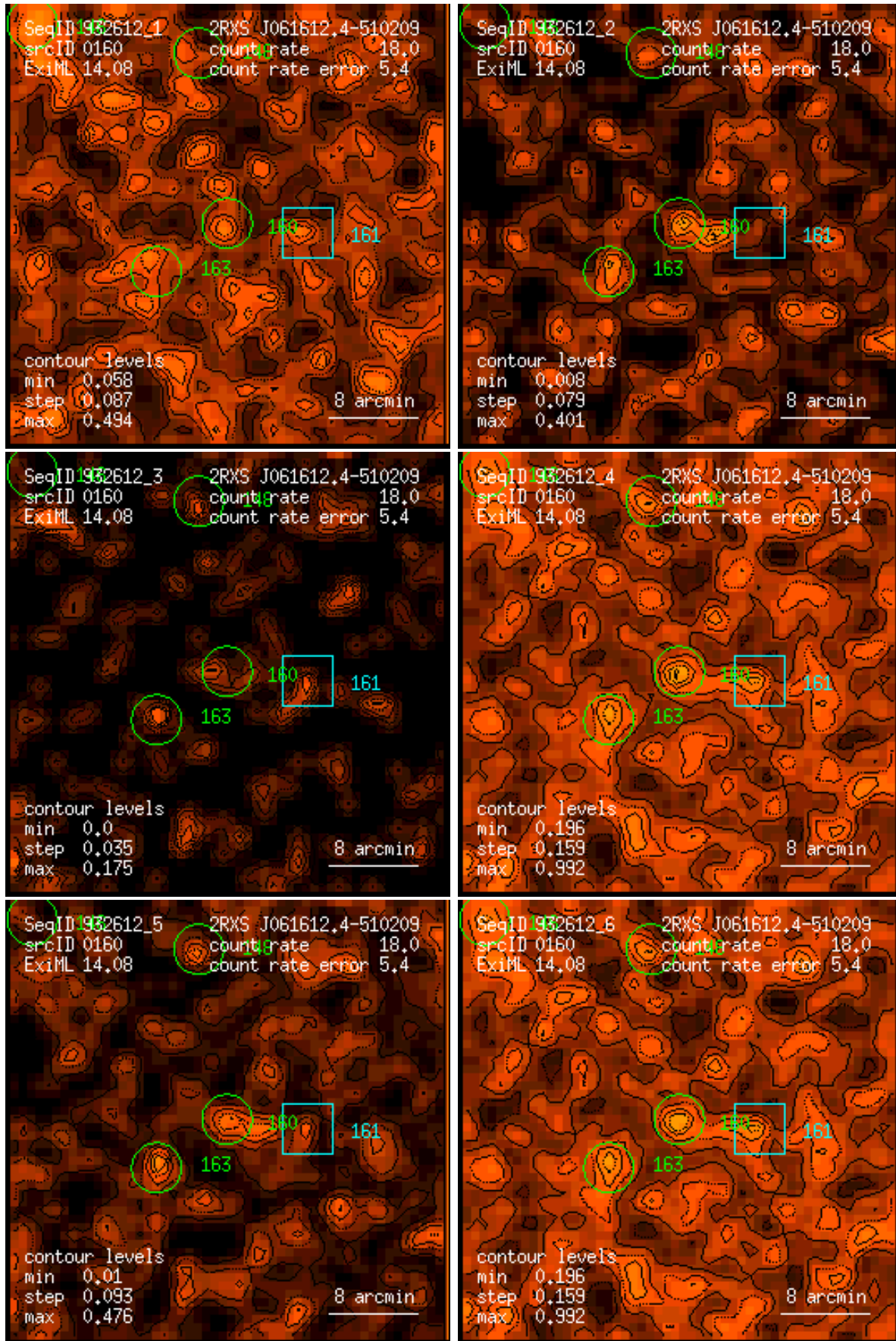
Figure 160: RASS 932612: detection 0160: band rate images, Gaussian filter: (1) PSPC channels 11 – 41, (2) 52 – 90, (3) 91 – 201, (4) 11 – 235, (5) 52 – 201, (6) 11 – 201. Broad band rates in counts/ks. Band rate contour levels in counts/ks/arcmin 2 .
