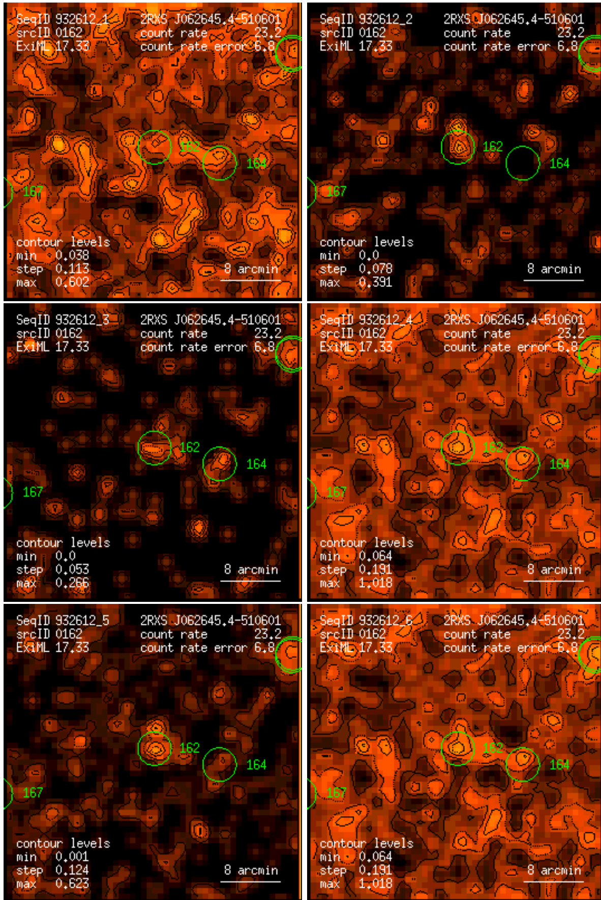
Figure 162: RASS 932612: detection 0162: band rate images, Gaussian filter: (1) PSPC channels 11 – 41, (2) 52 – 90, (3) 91 – 201, (4) 11 – 235, (5) 52 – 201, (6) 11 – 201. Broad band rates in counts/ks. Band rate contour levels in counts/ks/arcmin 2 .
