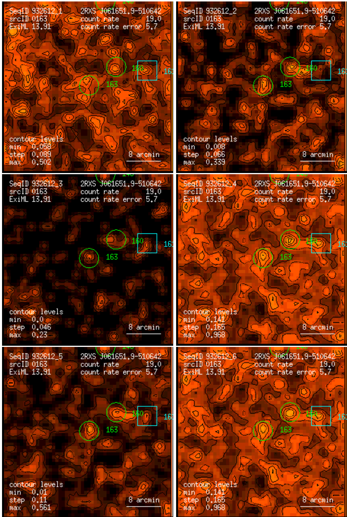
Figure 163: RASS 932612: detection 0163: band rate images, Gaussian filter: (1) PSPC channels 11 – 41, (2) 52 – 90, (3) 91 – 201, (4) 11 – 235, (5) 52 – 201, (6) 11 – 201. Broad band rates in counts/ks. Band rate contour levels in counts/ks/arcmin 2 .
