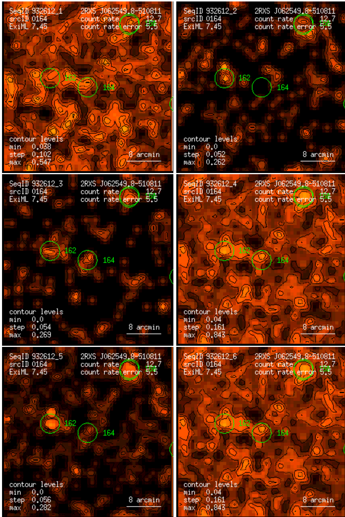
Figure 164: RASS 932612: detection 0164: band rate images, Gaussian filter: (1) PSPC channels 11 – 41, (2) 52 – 90, (3) 91 – 201, (4) 11 – 235, (5) 52 – 201, (6) 11 – 201. Broad band rates in counts/ks. Band rate contour levels in counts/ks/arcmin 2 .
