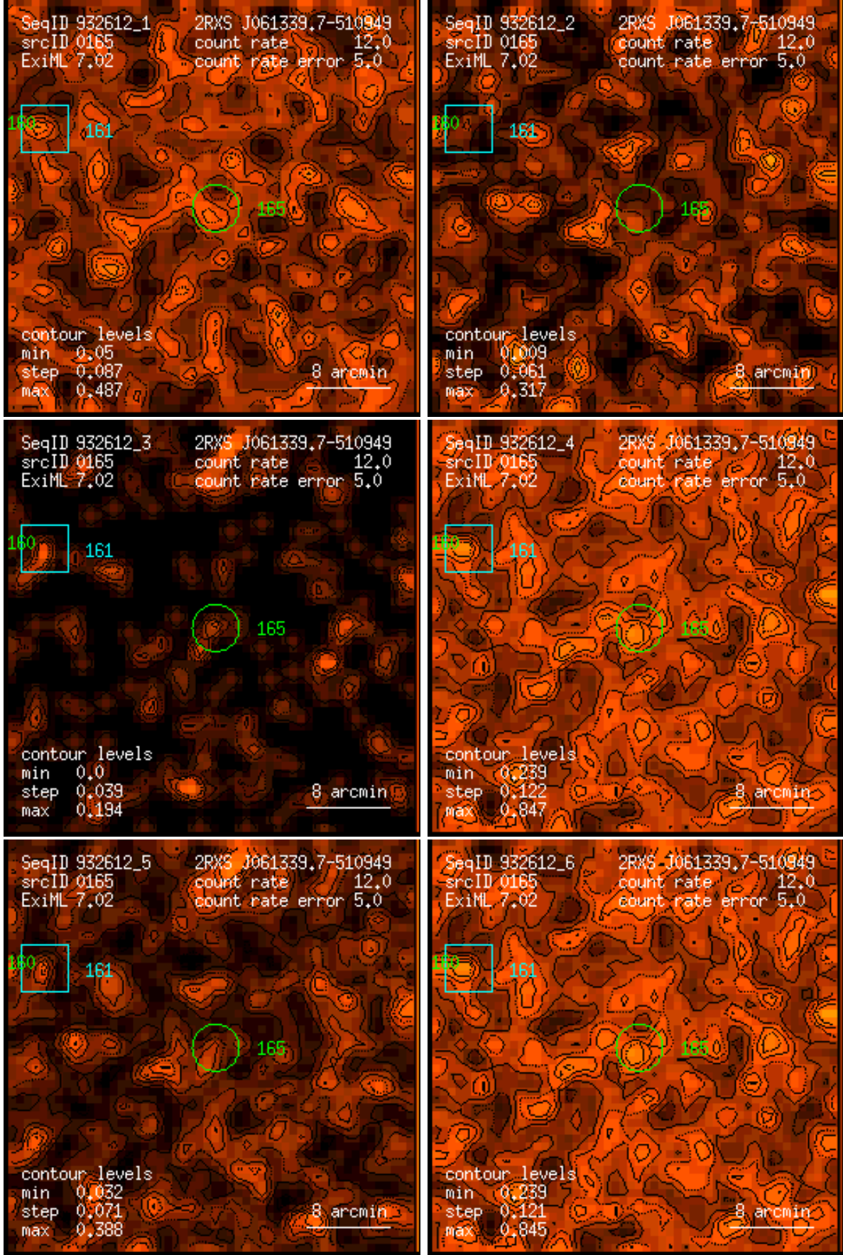
Figure 165: RASS 932612: detection 0165: band rate images, Gaussian filter: (1) PSPC channels 11 – 41, (2) 52 – 90, (3) 91 – 201, (4) 11 – 235, (5) 52 – 201, (6) 11 – 201. Broad band rates in counts/ks. Band rate contour levels in counts/ks/arcmin 2 .
