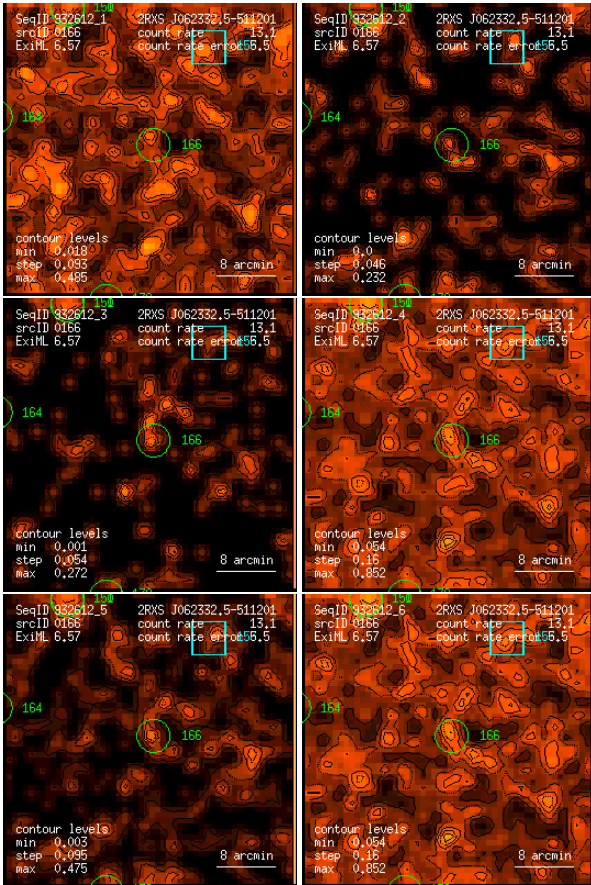
Figure 166: RASS 932612: detection 0166: band rate images, Gaussian filter: (1) PSPC channels 11 – 41, (2) 52 – 90, (3) 91 – 201, (4) 11 – 235, (5) 52 – 201, (6) 11 – 201. Broad band rates in counts/ks. Band rate contour levels in counts/ks/arcmin 2 .
