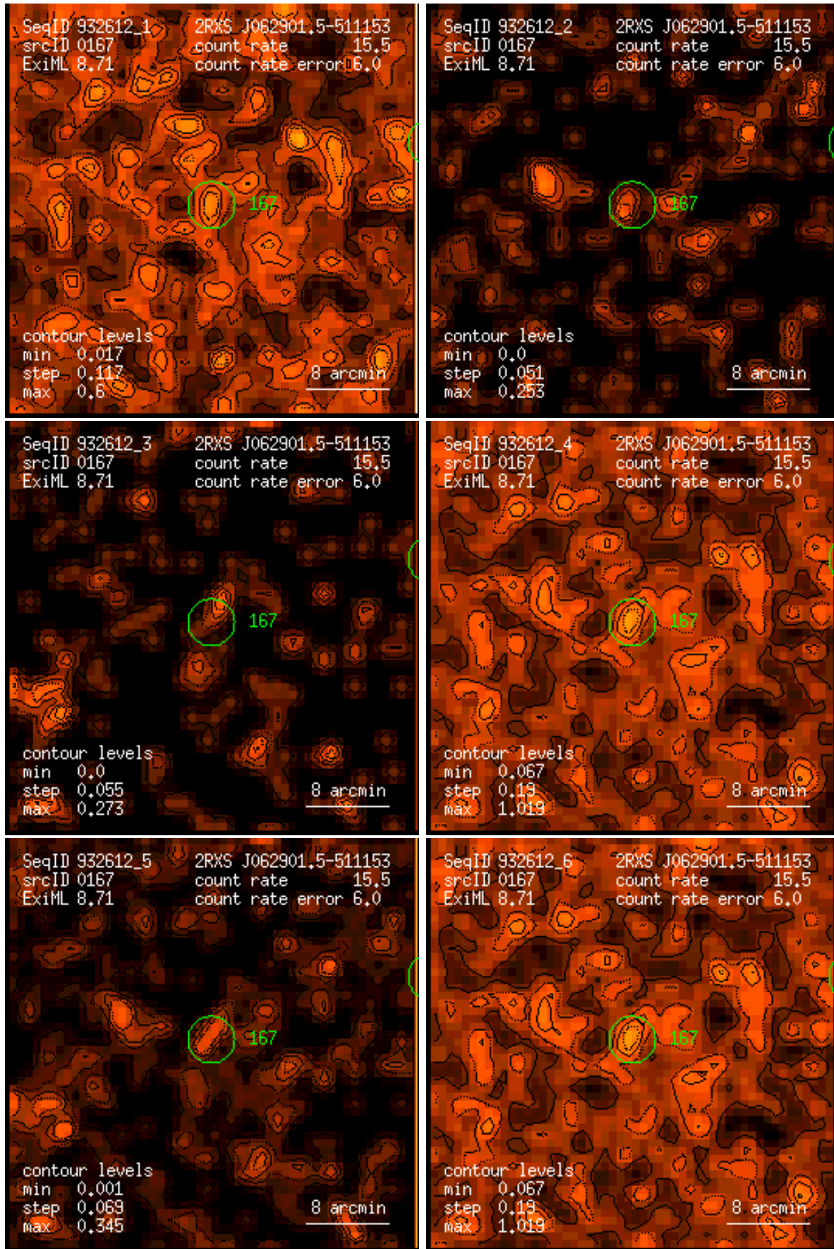
Figure 167: RASS 932612: detection 0167: band rate images, Gaussian filter: (1) PSPC channels 11 – 41, (2) 52 – 90, (3) 91 – 201, (4) 11 – 235, (5) 52 – 201, (6) 11 – 201. Broad band rates in counts/ks. Band rate contour levels in counts/ks/arcmin 2 .
