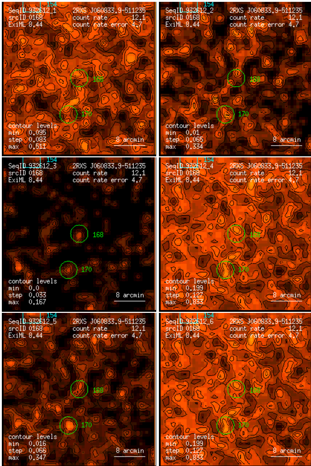
Figure 168: RASS 932612: detection 0168: band rate images, Gaussian filter: (1) PSPC channels 11 – 41, (2) 52 – 90, (3) 91 – 201, (4) 11 – 235, (5) 52 – 201, (6) 11 – 201. Broad band rates in counts/ks. Band rate contour levels in counts/ks/arcmin 2 .
