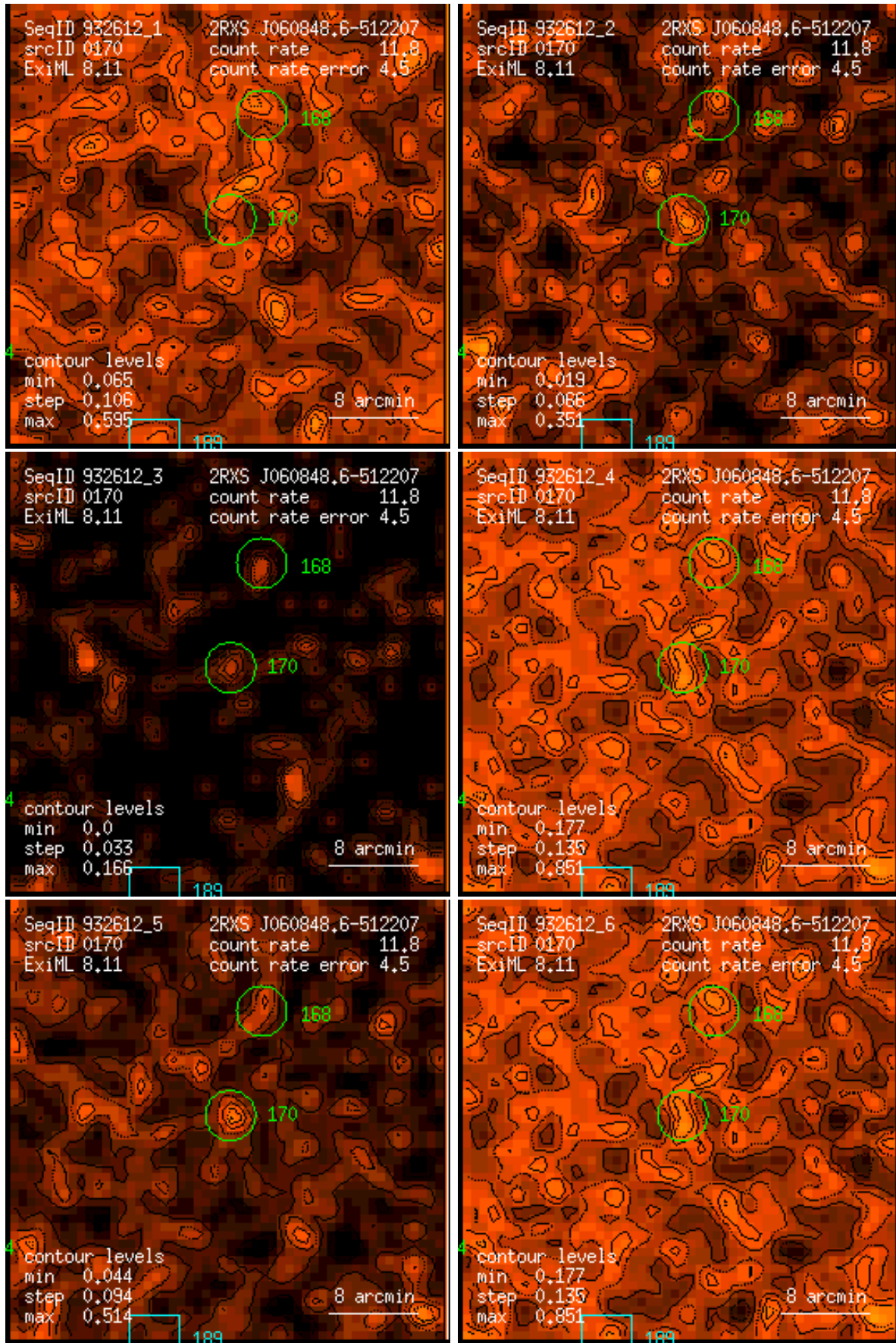
Figure 170: RASS 932612: detection 0170: band rate images, Gaussian filter: (1) PSPC channels 11 – 41, (2) 52 – 90, (3) 91 – 201, (4) 11 – 235, (5) 52 – 201, (6) 11 – 201. Broad band rates in counts/ks. Band rate contour levels in counts/ks/arcmin 2 .
