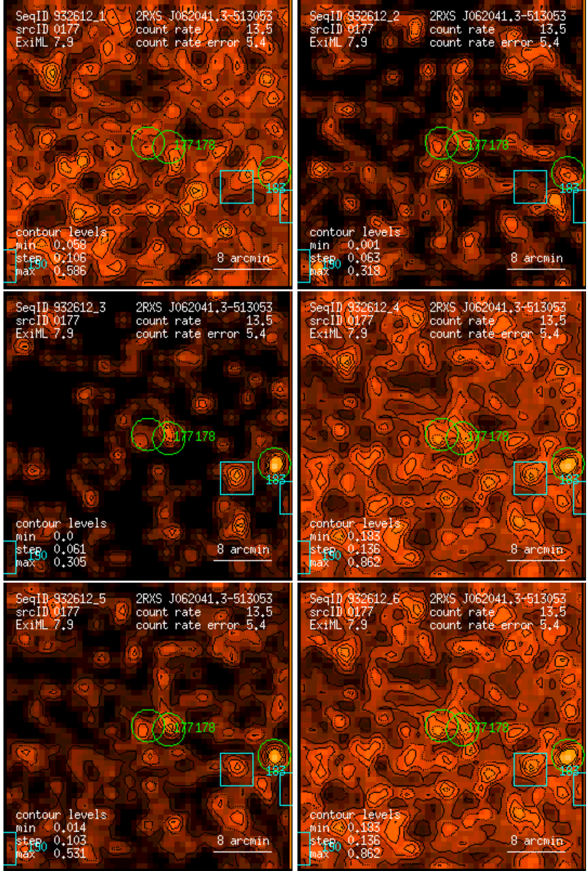
Figure 177: RASS 932612: detection 0177: band rate images, Gaussian filter: (1) PSPC channels 11 – 41, (2) 52 – 90, (3) 91 – 201, (4) 11 – 235, (5) 52 – 201, (6) 11 – 201. Broad band rates in counts/ks. Band rate contour levels in counts/ks/arcmin 2 .
