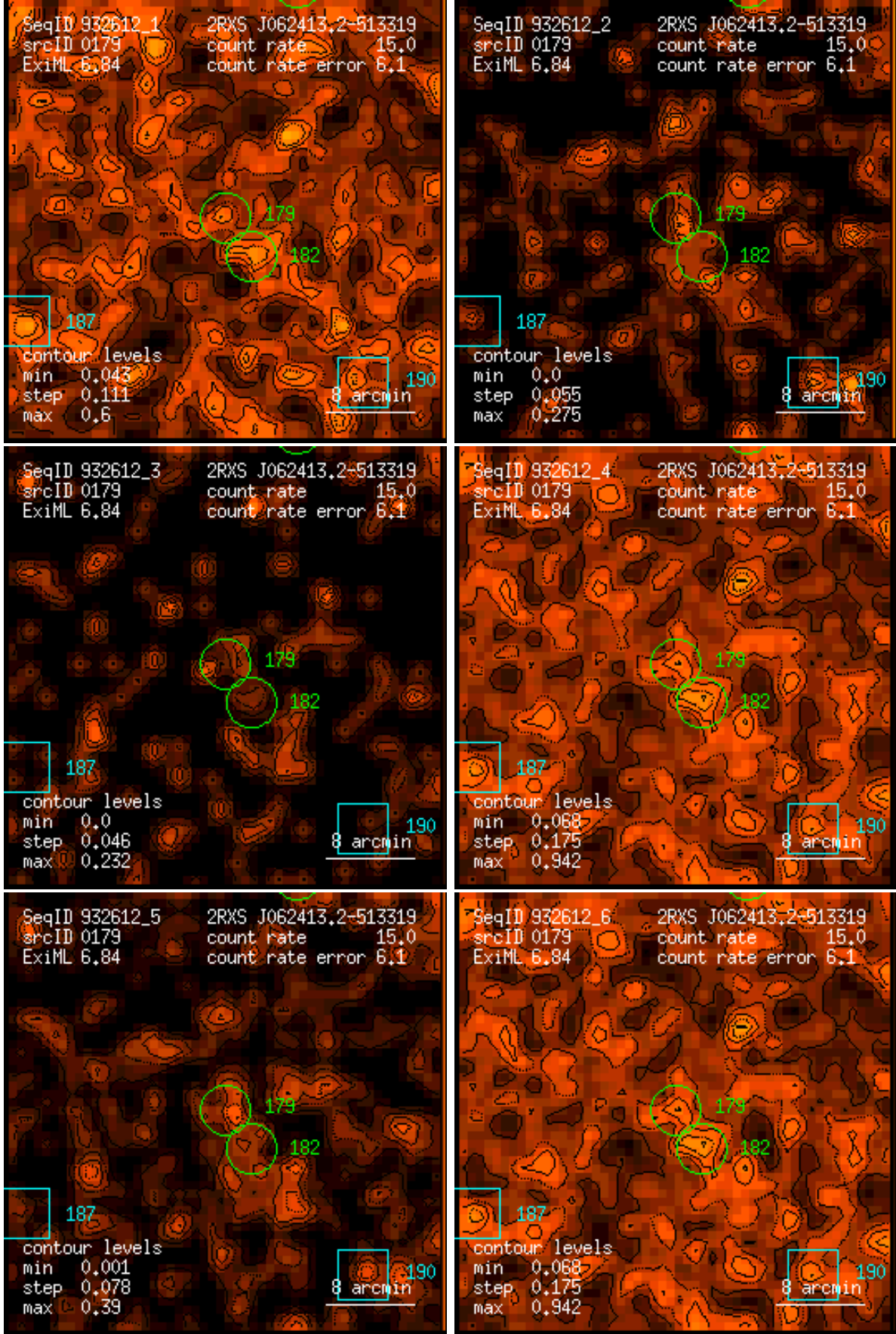
Figure 179: RASS 932612: detection 0179: band rate images, Gaussian filter: (1) PSPC channels 11 – 41, (2) 52 – 90, (3) 91 – 201, (4) 11 – 235, (5) 52 – 201, (6) 11 – 201. Broad band rates in counts/ks. Band rate contour levels in counts/ks/arcmin 2 .
