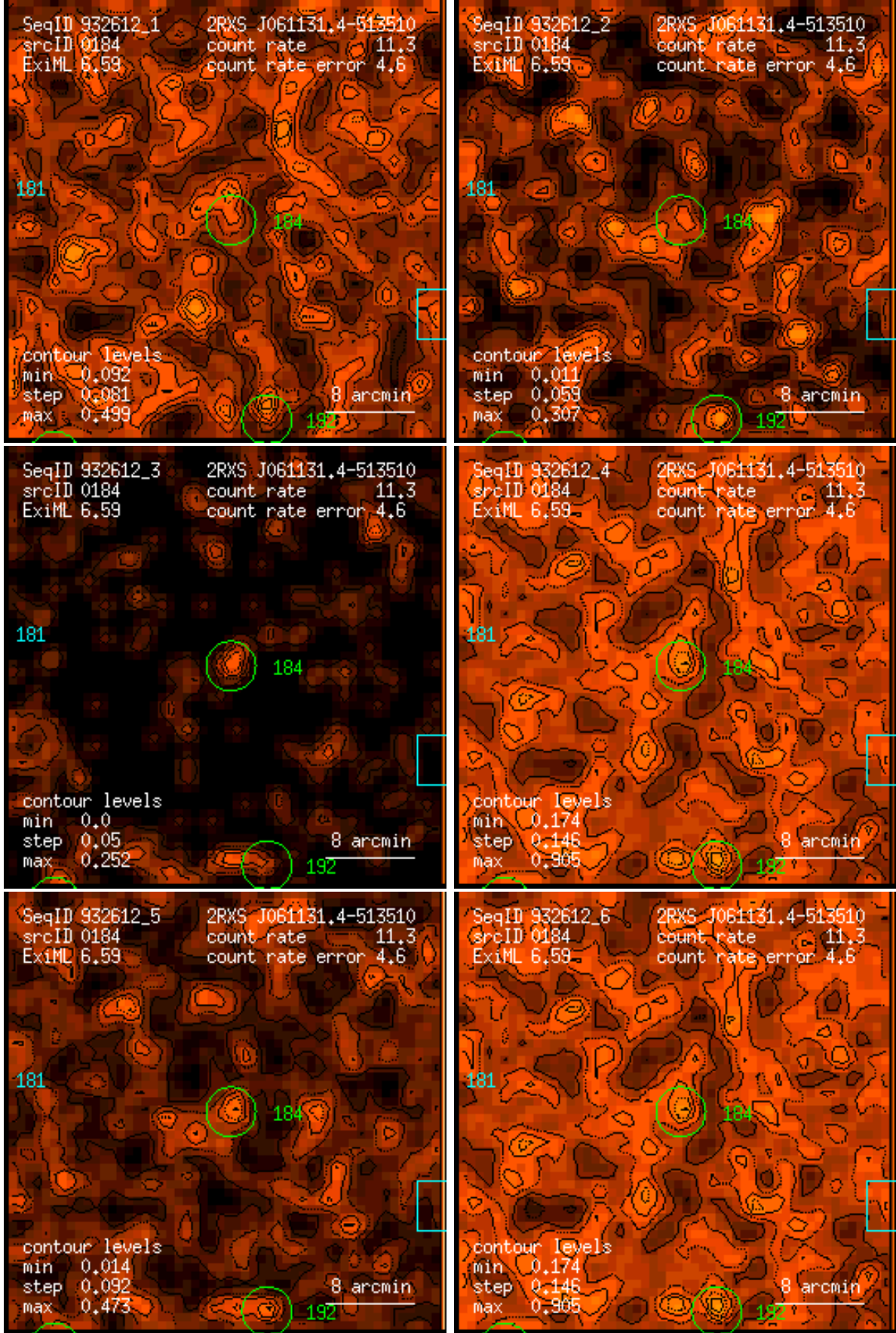
Figure 184: RASS 932612: detection 0184: band rate images, Gaussian filter: (1) PSPC channels 11 – 41, (2) 52 – 90, (3) 91 – 201, (4) 11 – 235, (5) 52 – 201, (6) 11 – 201. Broad band rates in counts/ks. Band rate contour levels in counts/ks/arcmin 2 .
