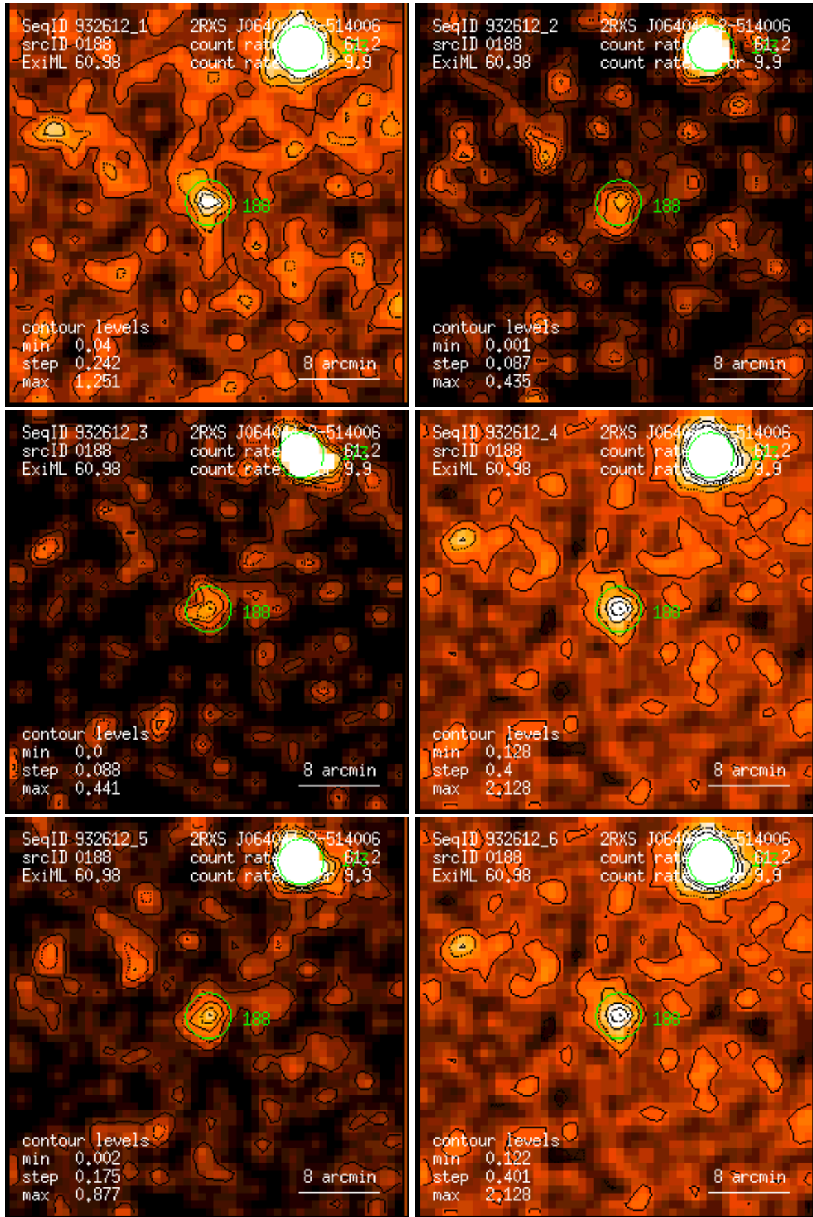
Figure 188: RASS 932612: detection 0188: band rate images, Gaussian filter: (1) PSPC channels 11 – 41, (2) 52 – 90, (3) 91 – 201, (4) 11 – 235, (5) 52 – 201, (6) 11 – 201. Broad band rates in counts/ks. Band rate contour levels in counts/ks/arcmin 2 .
