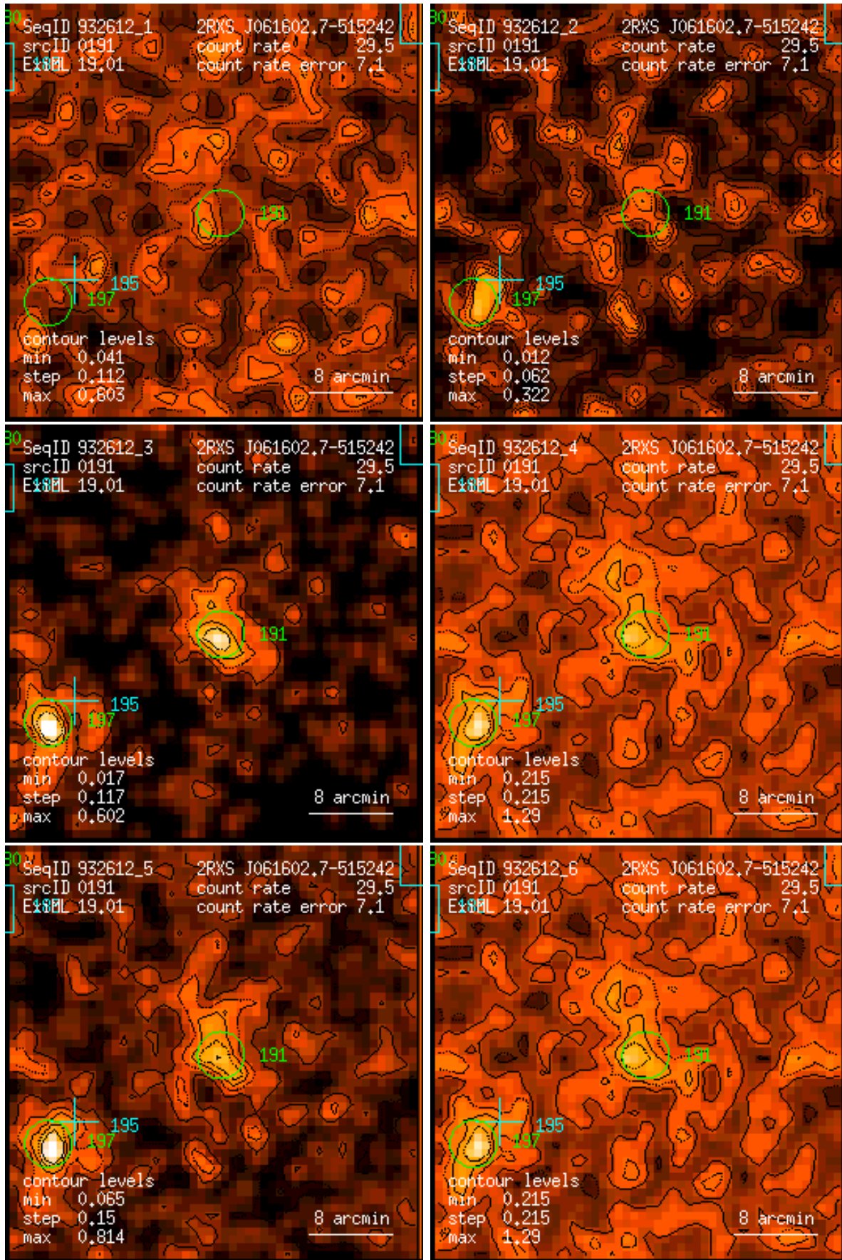
Figure 191: RASS 932612: detection 0191: band rate images, Gaussian filter: (1) PSPC channels 11 – 41, (2) 52 – 90, (3) 91 – 201, (4) 11 – 235, (5) 52 – 201, (6) 11 – 201. Broad band rates in counts/ks. Band rate contour levels in counts/ks/arcmin 2 .
