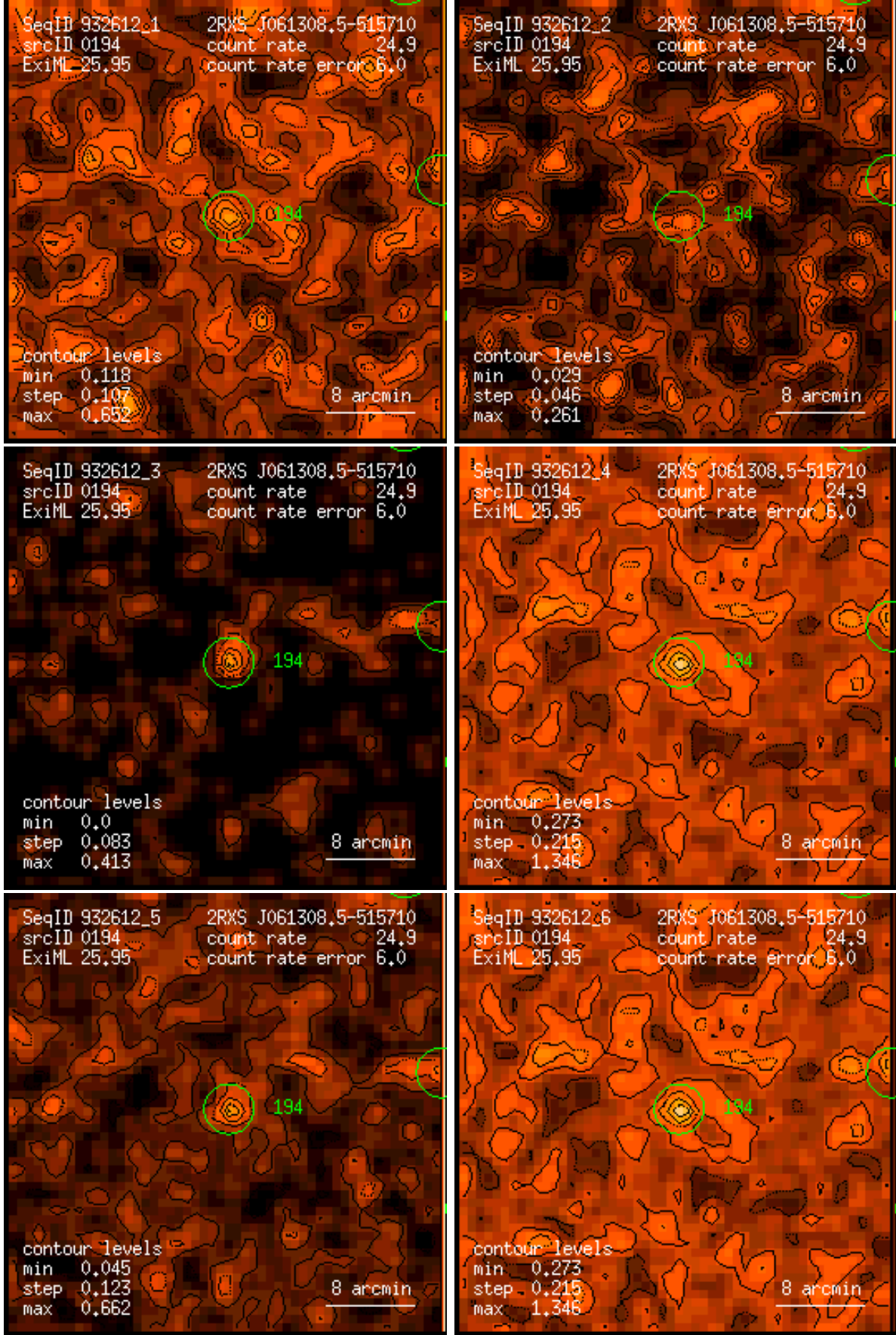
Figure 194: RASS 932612: detection 0194: band rate images, Gaussian filter: (1) PSPC channels 11 – 41, (2) 52 – 90, (3) 91 – 201, (4) 11 – 235, (5) 52 – 201, (6) 11 – 201. Broad band rates in counts/ks. Band rate contour levels in counts/ks/arcmin 2 .
