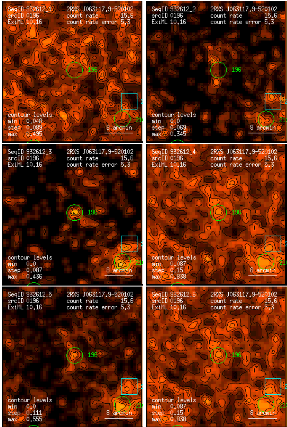
Figure 196: RASS 932612: detection 0196: band rate images, Gaussian filter: (1) PSPC channels 11 – 41, (2) 52 – 90, (3) 91 – 201, (4) 11 – 235, (5) 52 – 201, (6) 11 – 201. Broad band rates in counts/ks. Band rate contour levels in counts/ks/arcmin 2 .
