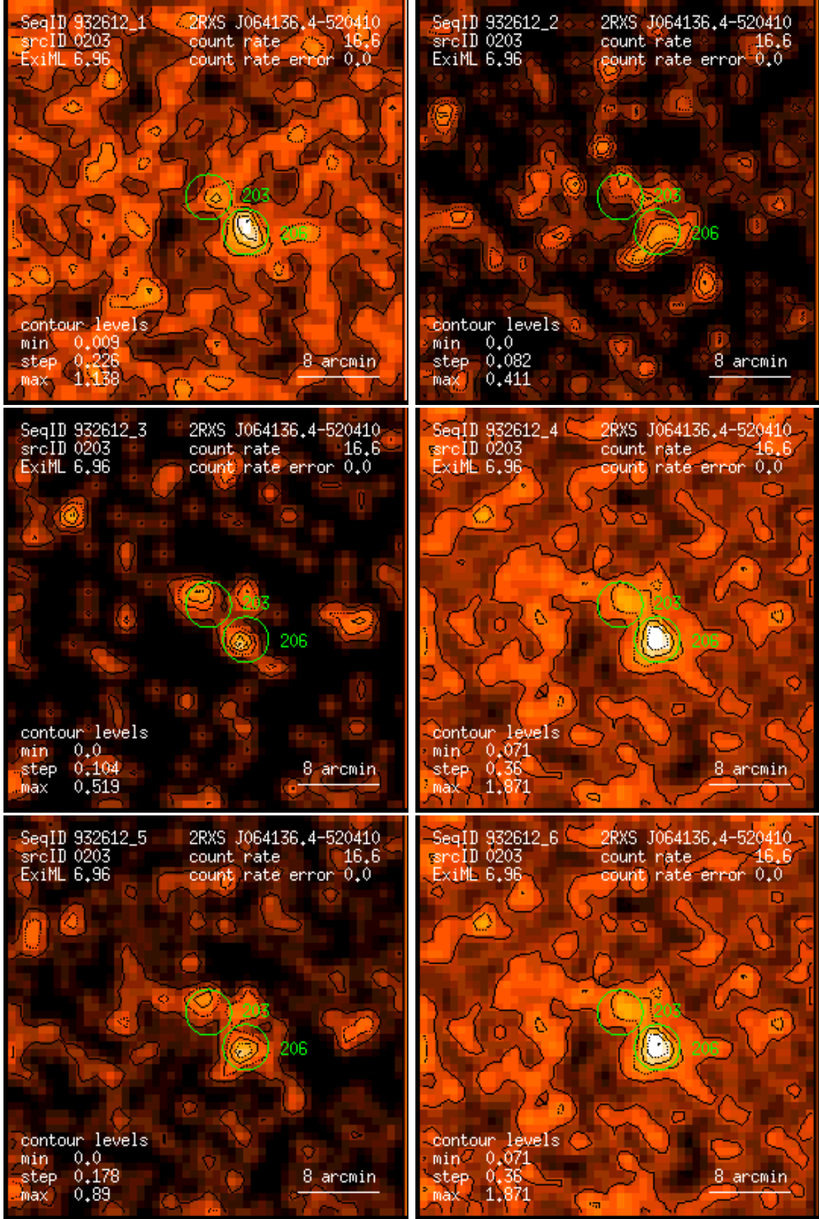
Figure 203: RASS 932612: detection 0203: band rate images, Gaussian filter: (1) PSPC channels 11 – 41, (2) 52 – 90, (3) 91 – 201, (4) 11 – 235, (5) 52 – 201, (6) 11 – 201. Broad band rates in counts/ks. Band rate contour levels in counts/ks/arcmin 2 .
