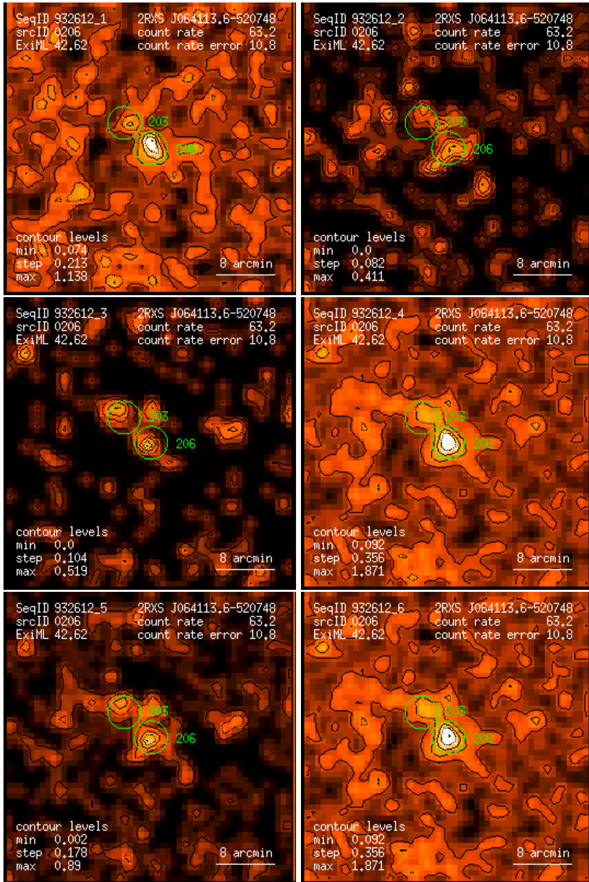
Figure 206: RASS 932612: detection 0206: band rate images, Gaussian filter: (1) PSPC channels 11 – 41, (2) 52 – 90, (3) 91 – 201, (4) 11 – 235, (5) 52 – 201, (6) 11 – 201. Broad band rates in counts/ks. Band rate contour levels in counts/ks/arcmin 2 .
