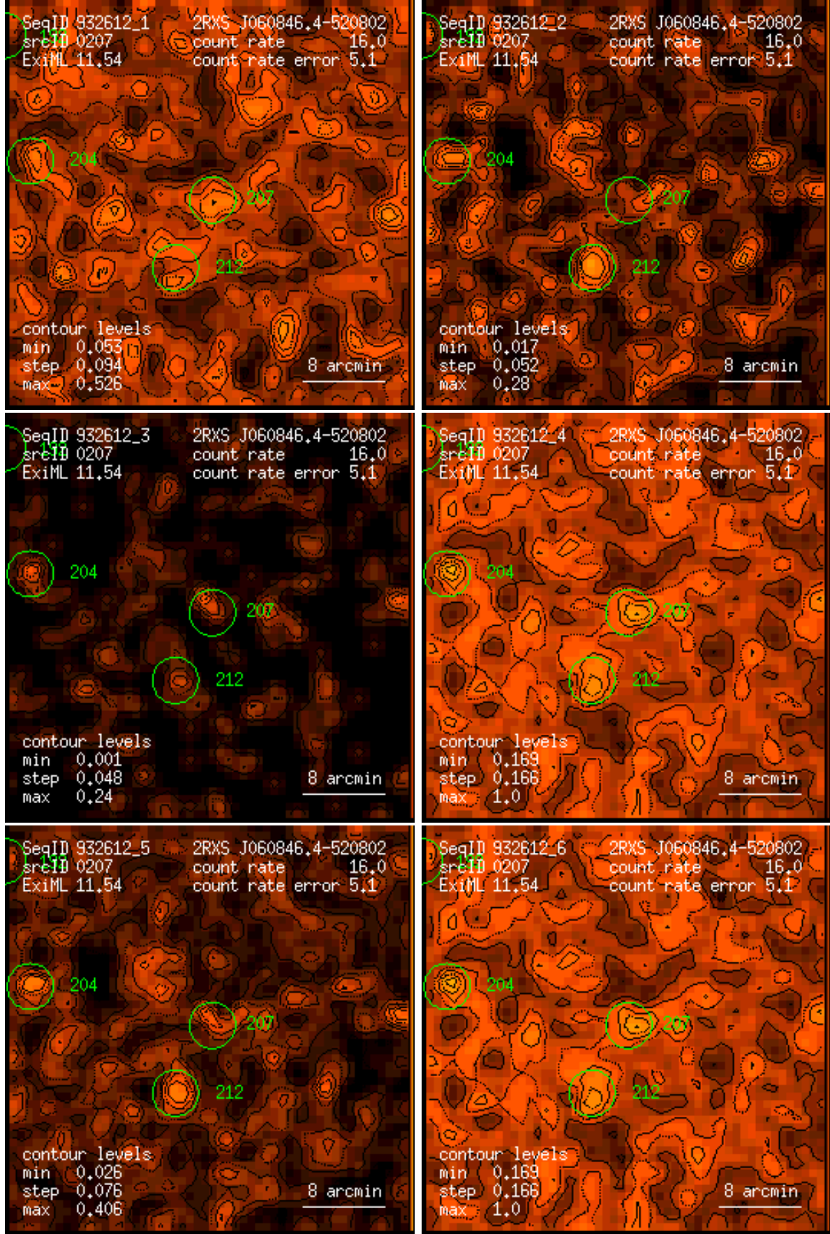
Figure 207: RASS 932612: detection 0207: band rate images, Gaussian filter: (1) PSPC channels 11 – 41, (2) 52 – 90, (3) 91 – 201, (4) 11 – 235, (5) 52 – 201, (6) 11 – 201. Broad band rates in counts/ks. Band rate contour levels in counts/ks/arcmin 2 .
