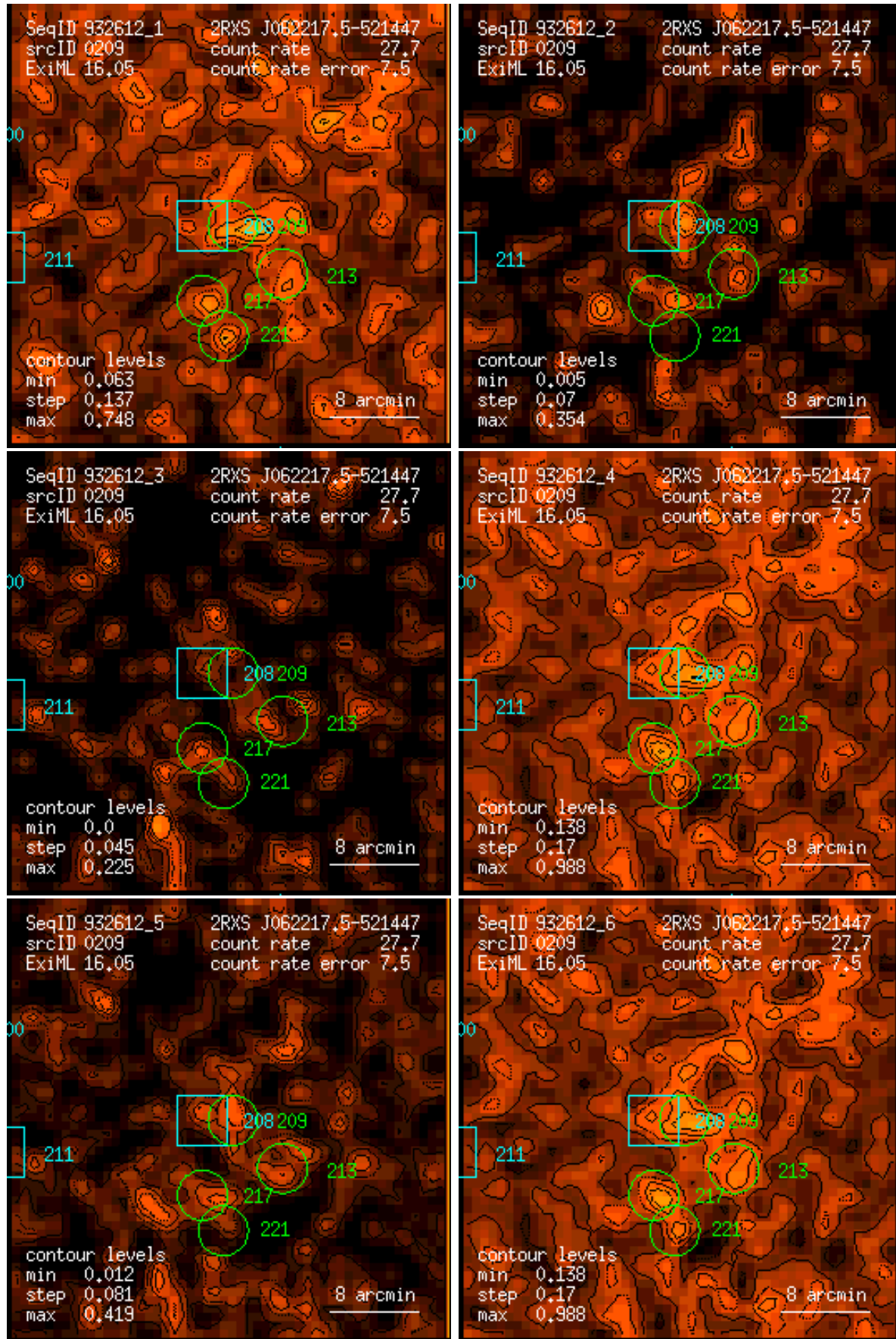
Figure 209: RASS 932612: detection 0209: band rate images, Gaussian filter: (1) PSPC channels 11 – 41, (2) 52 – 90, (3) 91 – 201, (4) 11 – 235, (5) 52 – 201, (6) 11 – 201. Broad band rates in counts/ks. Band rate contour levels in counts/ks/arcmin 2 .
